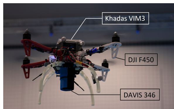
Fig. 2: Aerial robot used in the experiments.
