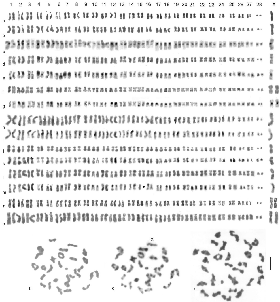
Figure 4. B. multilineatus – mitotic chromosomes from midgut and testis ( a–o ), metaphase I of meiosis, from testis ( p–r ) a ♂, Sweden, Åmsele, plain (Giemsa stained), shown as fig. 2o by Dutton and Angus (2007) b, c ♂, Scotland, Clatteringshaws Loch b plain c C-banded d–g France, Hautes-Pyrénées, Lac d’Oncet d, e ♂ f, g ♀ d, f plain e, g C-banded, shown as fig. 3g–j by Angus (2010b) h, i ♂, France, Hautes-Pyrénées, Lac d’Anapéou h plain i C-banded, shown as fig. 5k, l by Angus et al. (2015) j ♂, France, Ariège, Etangs de Fontargente, plain k ♂, Spain, Ibon de Anayet Este l, m ♂, Spain, Ibon de Urdecito l plain m C-banded; One replicate of C-banded autosome 15 has been lost from m ; n ♀, Ireland, Antrim, Garron Plateau above Glen Arrif o ♀, Ireland, Cork, NW Bonane p, q metaphase I, Spain, Provincia de Huesca, Ibones de Urdicito o plain p C-banded r Ireland, Cork, NW Bonane, Metaphase I, plain. Scale bar: 5 μm.
