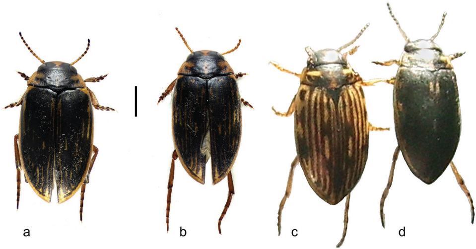
Figure 3. B. multilineatus and griseostriatus , habitus a, b multilineatus , Ireland, county Cork a ♀ b ♂ c B. griseostriatus , Switzerland, Le Louché d B. griseostriatus var. nigrescens Favre, Switzerland, Le Louché. Scale bar: 1 mm for (a, b) ; c, d are field photographs by Dr E. M. Angus.
