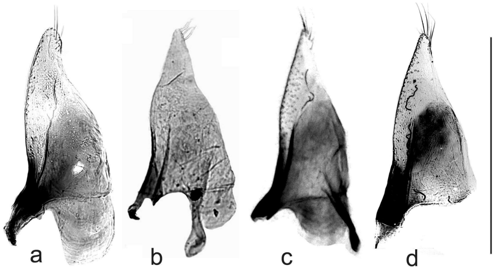
Figure 8. Boreonectes parameres. a B. multilineatus , Ireland, county Cork b–d B. griseostriatus b Starunia fossil c Norway, Tjøme d Sweden, Öregrund. The apodeme on the inner face is present in b and c but lost from a and d ; d also lacks the basal lobe. Scale bar: 0.5 mm.
