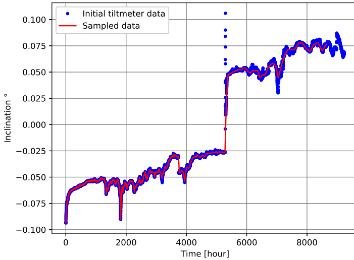
FIGURE 11 Comparison of initial dataset obtained under constant sampling rate of 1 hour with a dataset obtained under DDASA (here initial tiltmeter data and sampled data respectively)
