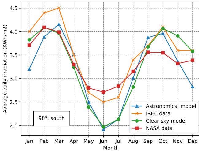
FIGURE 4 Comparison of average daily irradiation for 90°
