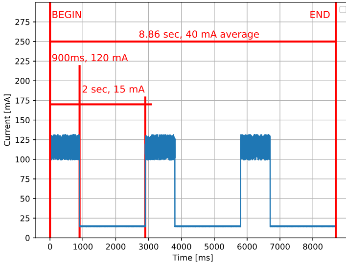
FIGURE 7 Radio consumption profile of LS device
