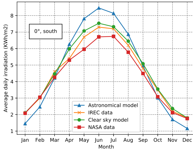
FIGURE 2 Comparison of average daily irradiation for 0°
