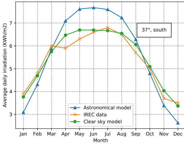
FIGURE 3 Comparison of average daily irradiation for 37°
