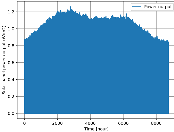
FIGURE 8 Theoretical power output of solar panel SOLEM 10/150/100 (south, 37°) located in Barcelona, Spain throughout a year.
