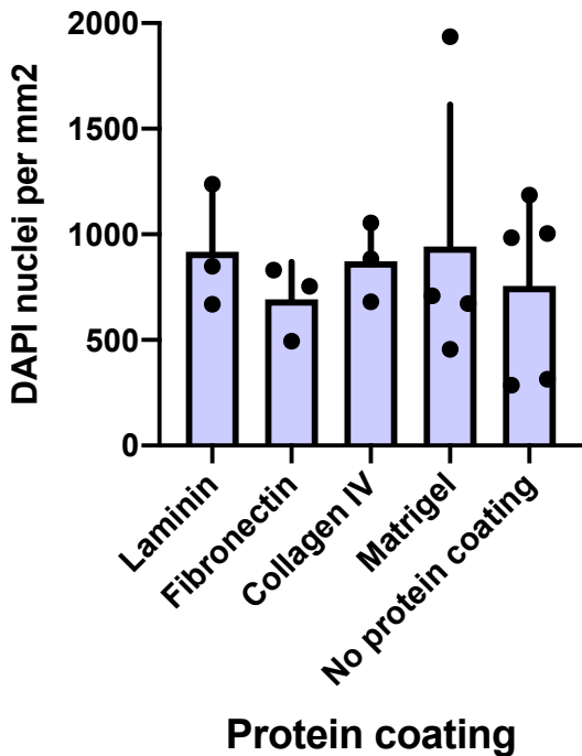
Fig S1a DAPI objects ECM proteins
