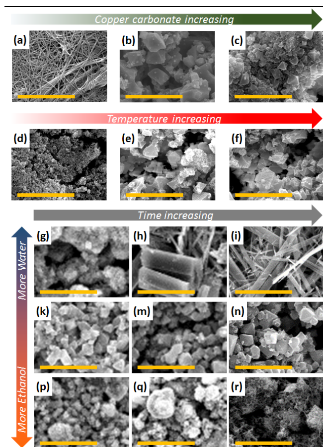
Figure 1 SEM micrographs of HKUST-1 MOF ( \text{Cu}_3\text{btc}_2 ) obtained from basic copper carbonate by conversion using 6.5 mL of \text{H}_3\text{btc} solution with (a-c) different amounts of copper carbonate (a: 20 mg, b: 200 mg, c: 2000 mg), (d-f) different temperatures (a: -78^\circ\text{C} , b: 24^\circ\text{C} , c: 80^\circ\text{C} ), and different amount of EtOH (g,h,i: 0% EtOH; k,m,n: 50% EtOH; p,q,r: 100% EtOH), with different reaction times (g,k,p: 20 minutes; h,m,q: 3 hours; i,n,r: 24 hours). For pictures a-f, the reaction time was three hours. Scalebar: 10\ \mu\text{m} (see Supplementary Information Figure S2-S4 for a complete survey).
