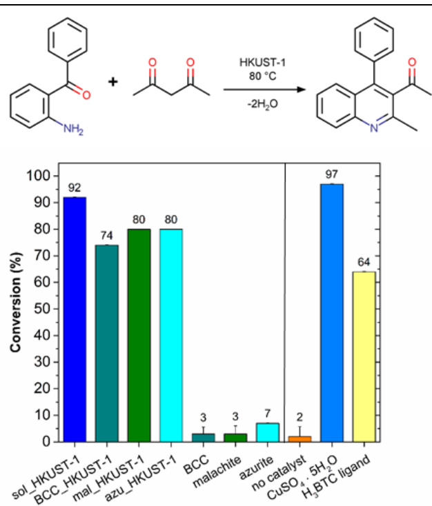
Figure 4. Catalytic performance in the Friedländer condensation between 2ABP and Acac (as percentage of quinoline produced from the aminophenone) of sol_HKUST-1 (blue, from solvothermal synthesis), BCC_HKUST-1 (teal, from basic copper carbonate), mal_HKUST-1 (green, from malachite), azu_HKUST-1 (cyan, from azurite), and their carbonate sources. The reaction was also performed without catalyst (orange), in presence of copper sulfate (light blue), or the H 3 BTC ligand (light yellow). Reaction conditions: 2ABP/Acac/HKUST-1 molar ratio: 5:1:0.083.
