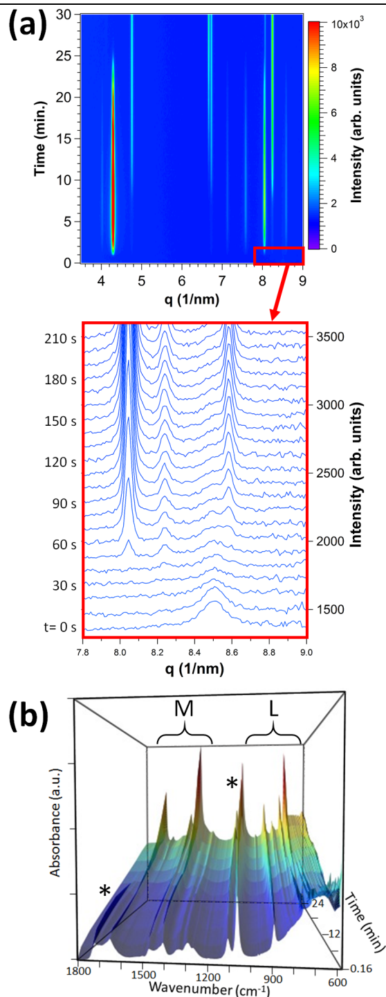
Figure 3. a) SAXS/WAXS kinetics in the first 30 minutes of reaction of the carbonate to HKUST-1. The magnification (red box) show the disappearance of the carbonate peak at 8.5 \text{ nm}^{-1} during the first minute of reaction, and the appearance of the intermediate peaks at 8.0 and 8.6 \text{ nm}^{-1} , and the (222) HKUST-1 peak at 8.2 \text{ nm}^{-1} ; b) FTIR kinetics in the first 24 minutes of conversion, with regions attributable to the metal sites and the ligands, respectively. The bands indicated with an asterisk (*) are associated to the residual intermediate material. Detailed FTIR spectra are available in Supplementary Figure S13.
