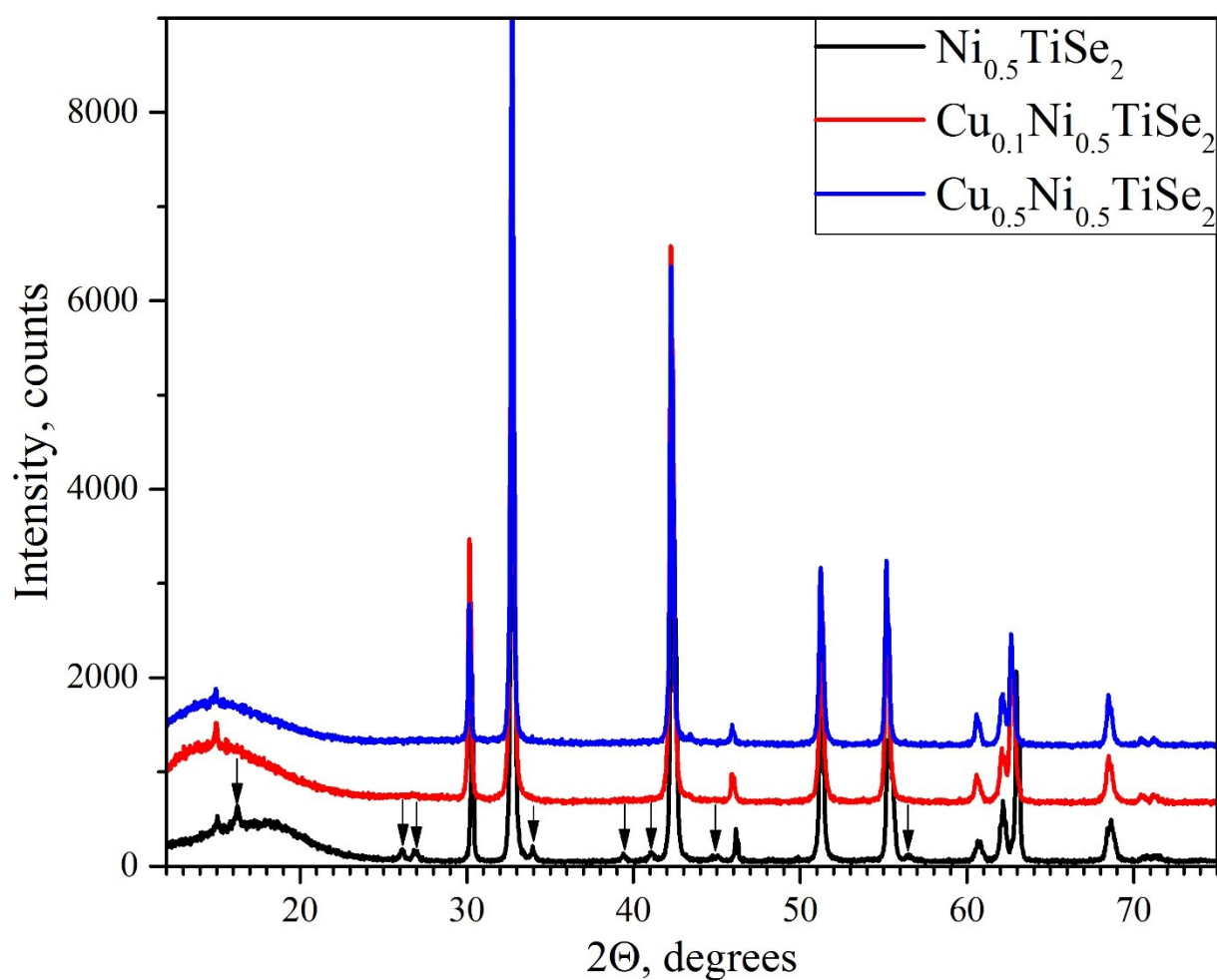
Figure s1. Diffraction patterns for \text{Cu}_x\text{Ni}_{0.5}\text{TiSe}_2 ( x=0, 0.1, 0.5 ). By arrows are indicated superstructure lines, which correspond to the a_0 \times \sqrt{3}a_0 \times 2c_0 super cell.
