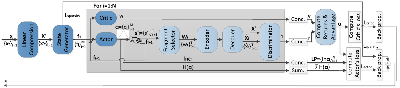
Fig. 4. The 4 th step of the incremental training procedure. Dark-coloured boxes denote the parts updated in this step.
