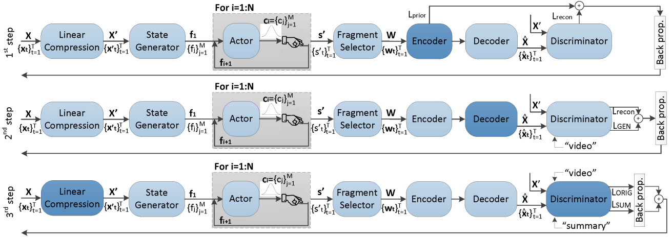
Fig. 3. The first three steps of the incremental training procedure. Dark-coloured boxes denote the parts updated in each step.
