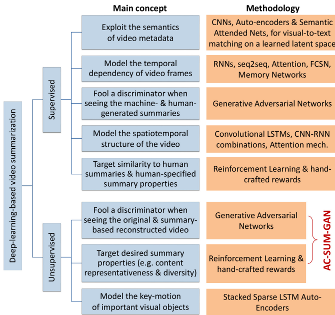
Fig. 1. A taxonomy of the current SoA methods for video summarization, and the positioning of the proposed AC-SUM-GAN method.
