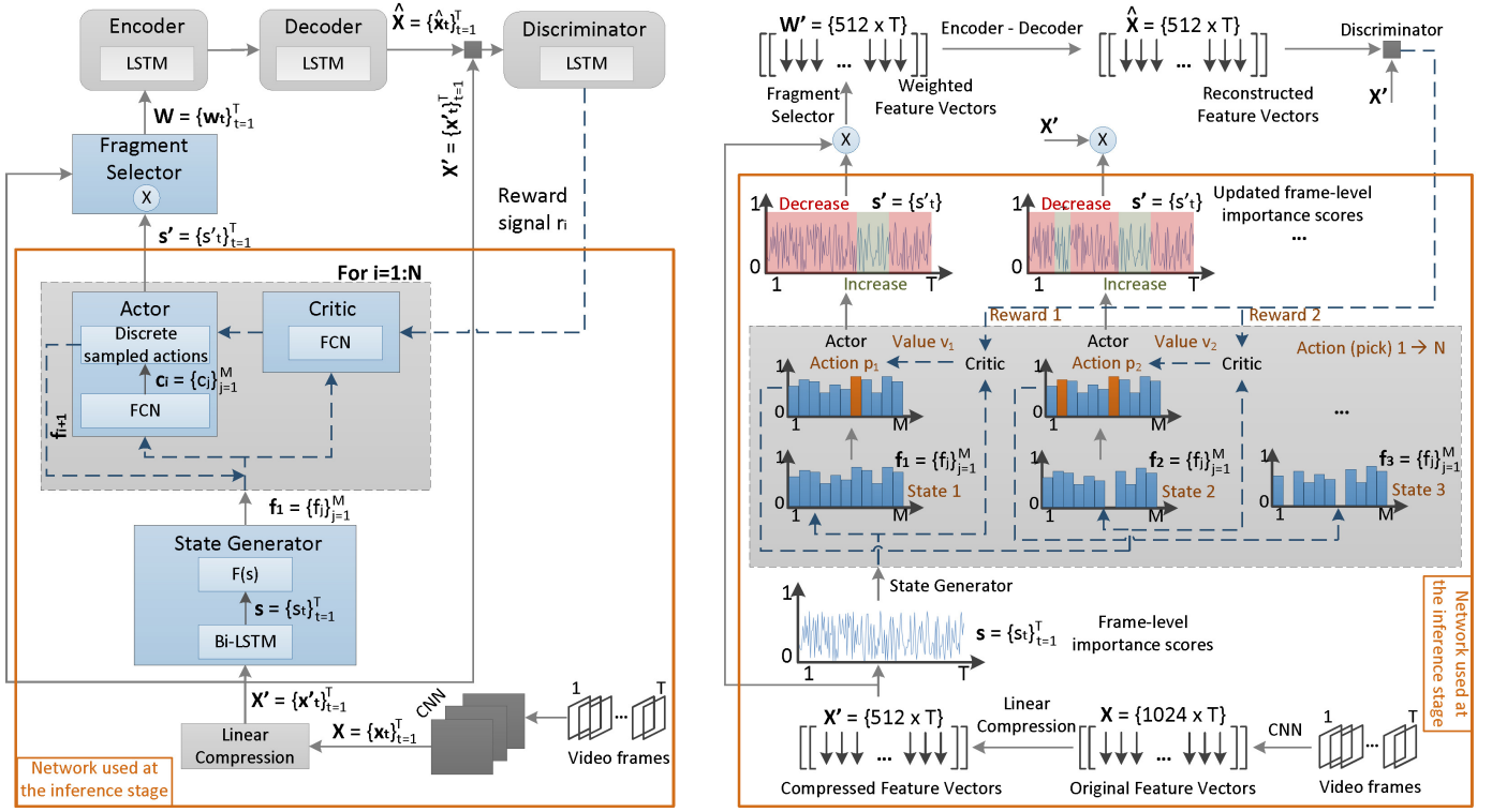
Fig. 2. The AC-SUM-GAN architecture. On the left side we show the building blocks of the architecture and their connections. Blue coloured rectangles indicate parts related to the Actor-Critic model. On the right side we give an example of the data flow by presenting the input and output of each different part of the architecture. On both sides of the figure, dashed lines represent iterative processes during the training of the AC part. The orange box shows the part of the architecture that is used for inference; at the training stage, the entire architecture is used.
