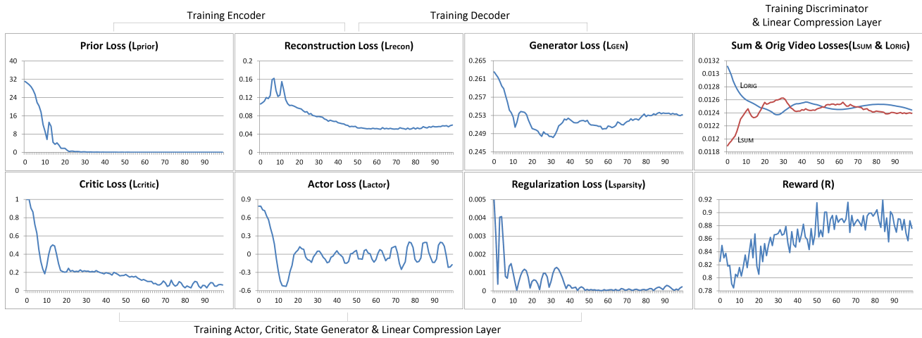
Fig. 5. Loss and reward curves for the proposed model. The horizontal axis in all plots indicates the epoch number. These curves indicate the successful training of Encoder, Decoder, Actor, Critic, State Generator and Discriminator, and the model’s ability to get higher rewards as the training proceeds.
