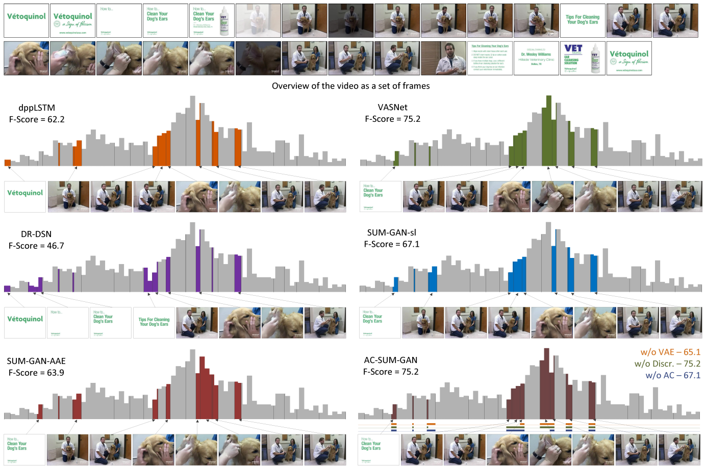
Fig. 7. A key-frame-based overview (using one key-frame per shot), and example summaries of six summarization methods on video #15 of the TVSum dataset (the first two methods, dppLSTM and VASNet, are supervised, while the rest are unsupervised). For AC-SUM-GAN, we also illustrate with coloured horizontal line segments under the corresponding bar-chart, the result of each of the three variations of it discussed in the ablation study (Section V-C).
