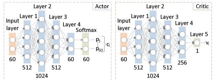
Fig. 6. The architecture of Actor and Critic models. The values below each layer’s sketch represent the size of the layer (number of nodes).
