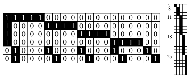
Figure 2: On the left the A_1 of the first case is shown. On the right the upper-left 25 \times 5 submatrix of its associated A_2 is shown with some of its row numbers in A —this submatrix is completely determined under the assumption that its rows are lexicographically ordered.
