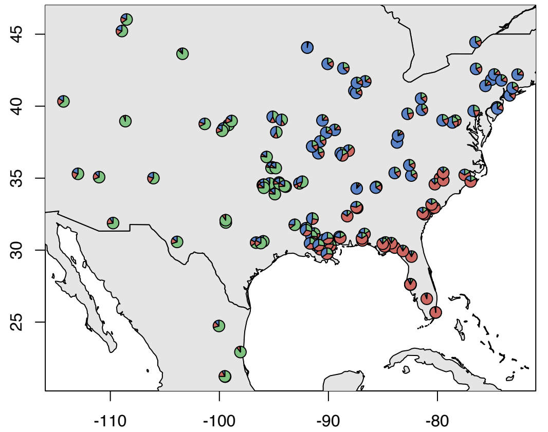
Missing = 0.45 Individuals = 144 Loci = 3389
