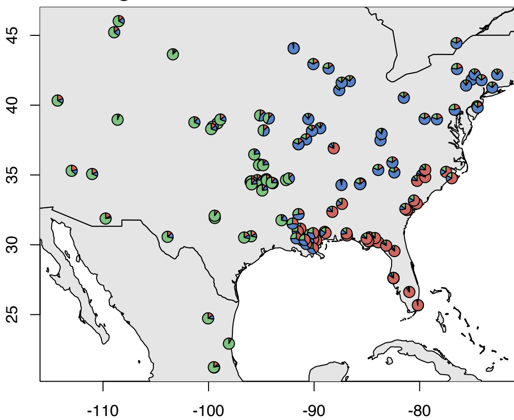
Missing = 0.39 Individuals = 129 Loci = 2473
