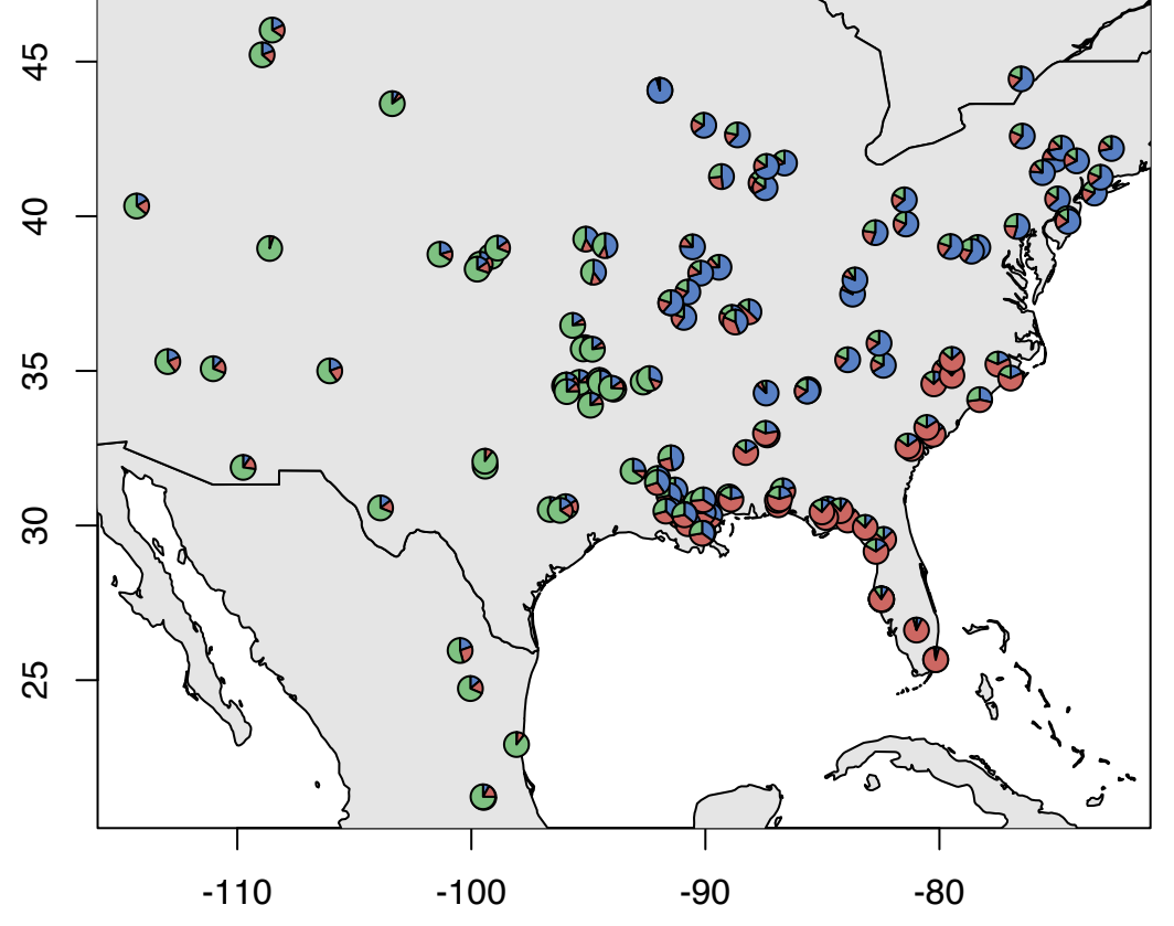
Missing = 0.46 Individuals = 150 Loci = 3391
