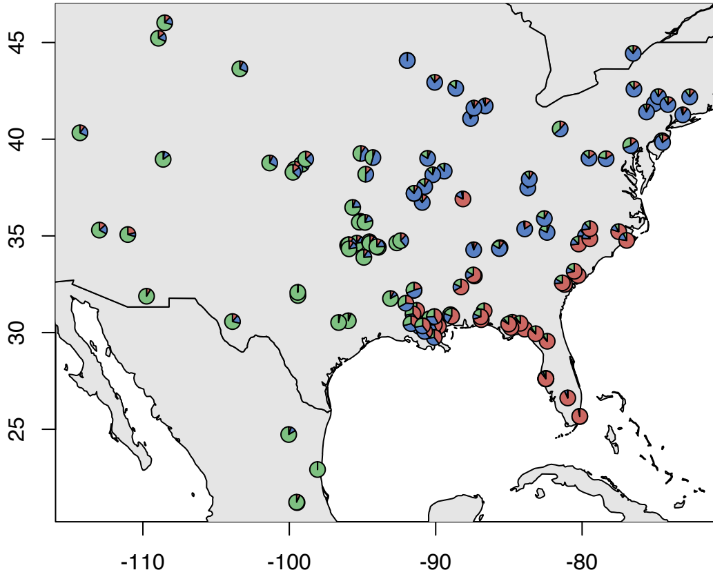
Missing = 0.29 Individuals = 132 Loci = 649
