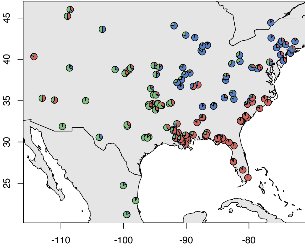
Missing = 0.19 Individuals = 145 Loci = 137
