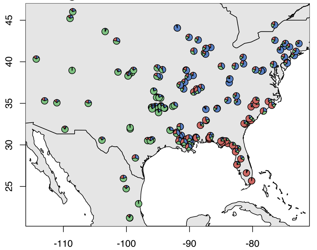
Missing = 0.48 Individuals = 159 Loci = 3391
