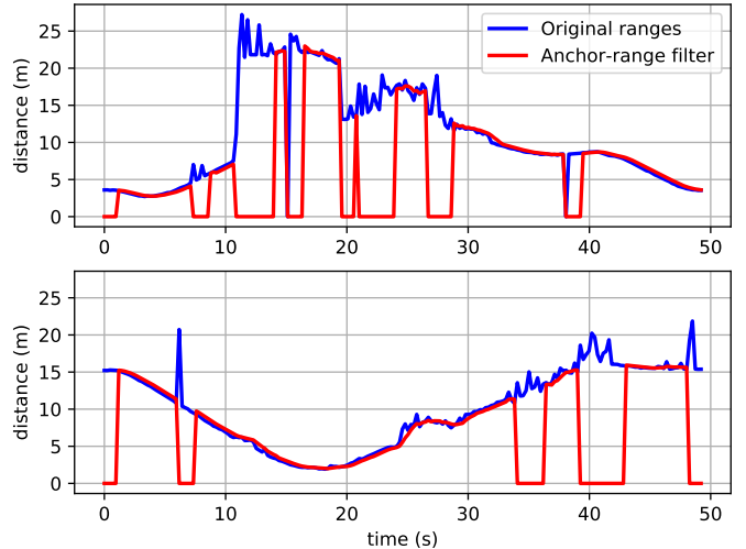
Fig. 2. Comparison between the distances provided by the Pozyx kit with regard to two different anchors and the outputs provided by our anchor-range filter. A 0-value indicates that the anchor is not available.
