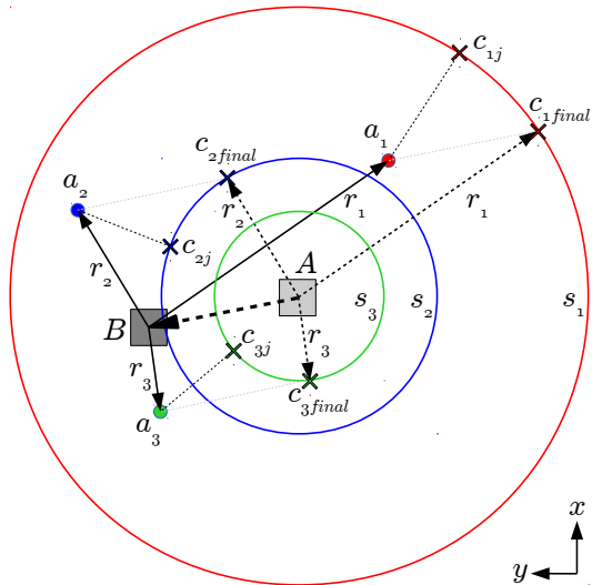
Fig. 1. Example of point-to-circumference correspondence when moving the tag from point A to B and for given anchors a_1 , a_2 and a_3 . c_{1j} , c_{2j} and c_{3j} are the closest points for the current iteration j . c_{1final} , c_{2final} and c_{3final} are the final correspondences after the ICP convergence.
