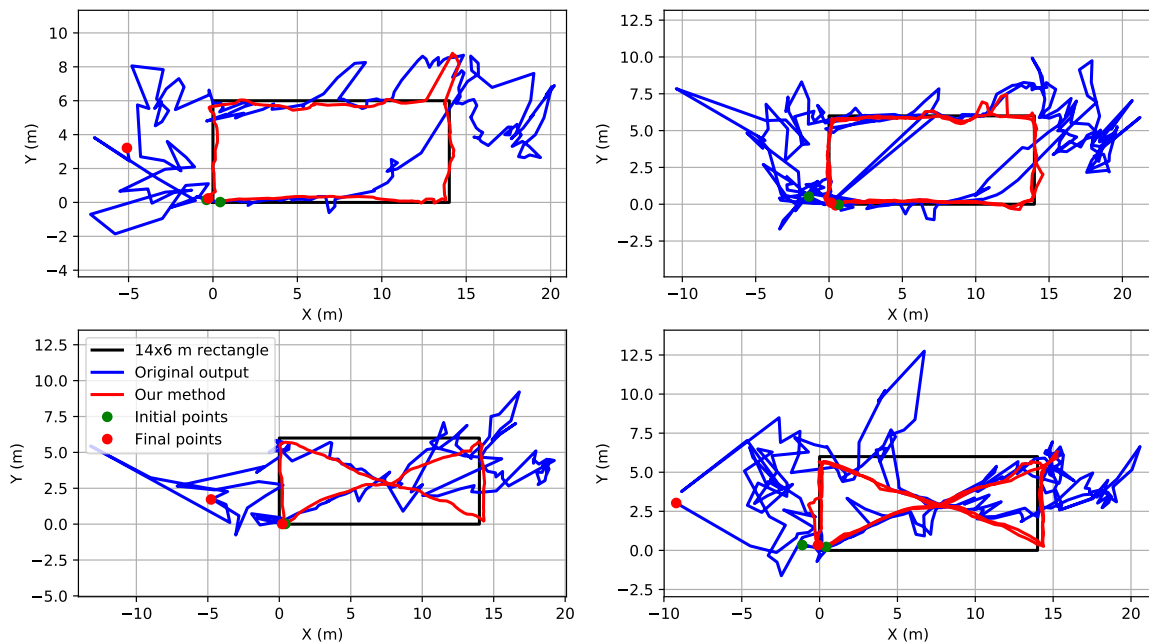
Fig. 3. Comparison between the outputs supplied by the Pozyx method and our approach when following four different trajectories. (top-left) rectangle-like trajectory, (top-right) rectangle-like trajectory \times 2 , (bottom-left) eight-like trajectory, and (bottom-right) eight-like trajectory \times 2 .
