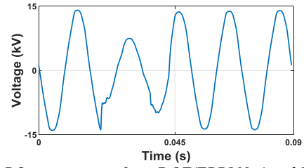
Fig. 2: PQ event extract from DOE/EPRI National Database.
