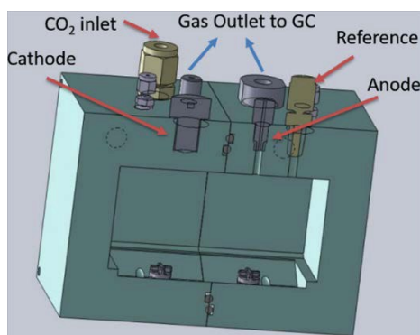
Figure 92. A schematic view of the electrochemical cell reported by Satre et al. Reprinted from 26 with the kind permission of John Willey and Sons. Copyright 2016.
