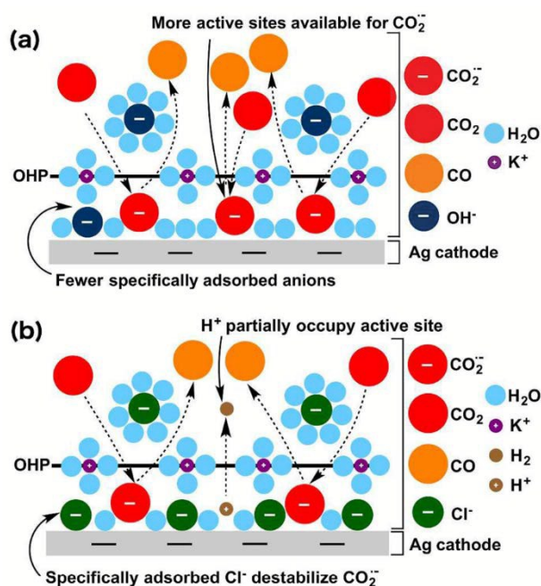
Figure 126. Schematic illustrations of processes in the double layer that play a role in the kinetics of \text{CO}_2 to \text{CO} conversion on a Ag cathode when using (a) KOH or (b) KCl as the electrolyte. Reproduced and adapted from 114 with the kind permission of the PCCP Owner Societies.
