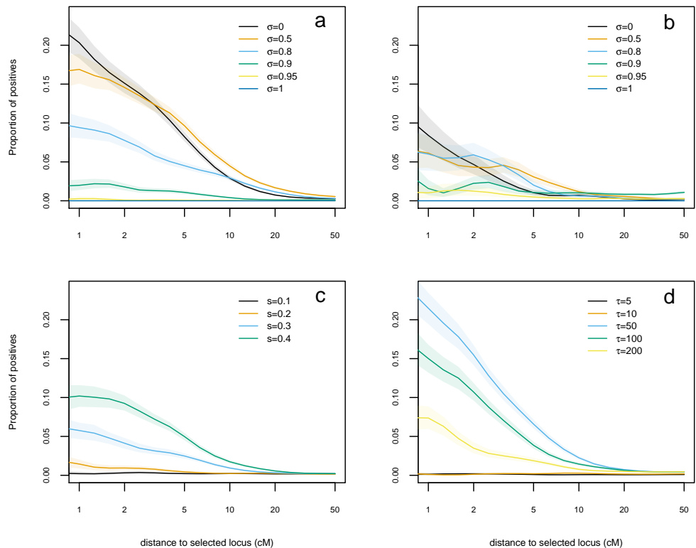
Figure 3. Selection footprint on the selected chromosome under different scenarios. Proportion of positive tests in function of distance to the locus under selection. Estimates obtained from 100 replicates of simulated data of one population of N = 500 diploid individuals, sampled twice with \tau generations between samples and selection coefficient s and selfing rate \sigma . (a) Adaptation from new mutation, \tau = 25 , s = 0.5 . (b) Adaptation from standing variation, \tau = 25 , s = 0.5 . (c) Adaptation from new mutation, \tau = 25 , \sigma = 0 . (d) Adaptation from new mutation, s = 0.5 , \sigma = 0 . Distance measured in centimorgans (cM). Coloured areas mark the 95% bootstrap interval.
