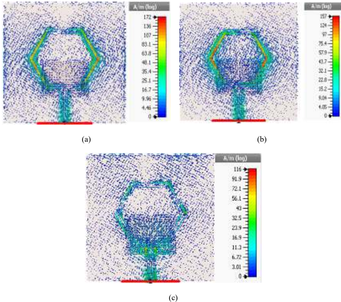
Figure 5. Simulated Surface current distribution, (a) 2.45 GHz, (b) 2.86, (c) 6.18 GHz
