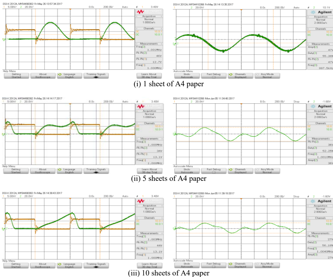
Figure 11. Series of diagrams indicating the outcomes of CPT system using zinc as the capacitive plates
