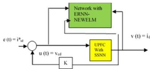
Figure 13. UPFC system presentation with state space and (ERNN-NEWELM)
