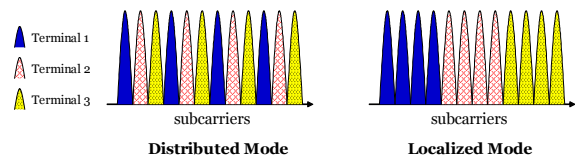
Figure 3 – Subcarrier allocation methods for multiple users ( Q=3 users, M=12 subcarriers, and N=4 subcarriers allocated per user).
