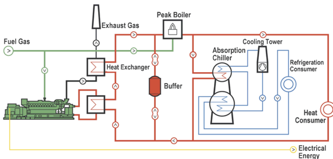
Figure 7: Trigeneration scheme [21]
