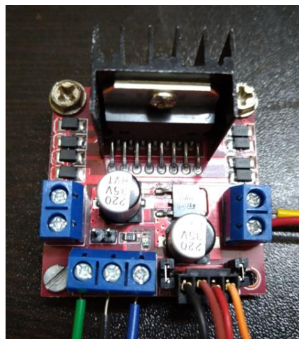
Figure 5. L298 DC motor driver board
