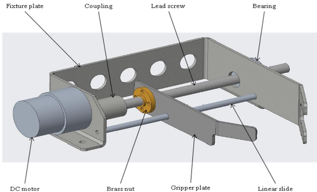
Figure 1. CAD assembly model of l.s.gripper
