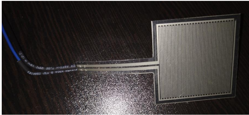
Figure 6. Force sensitive resistor, 40x40 mm area
