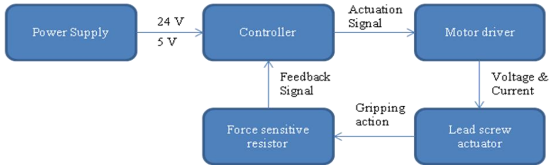
Figure 4. Mechatronic system concept for the l.s.gripper
