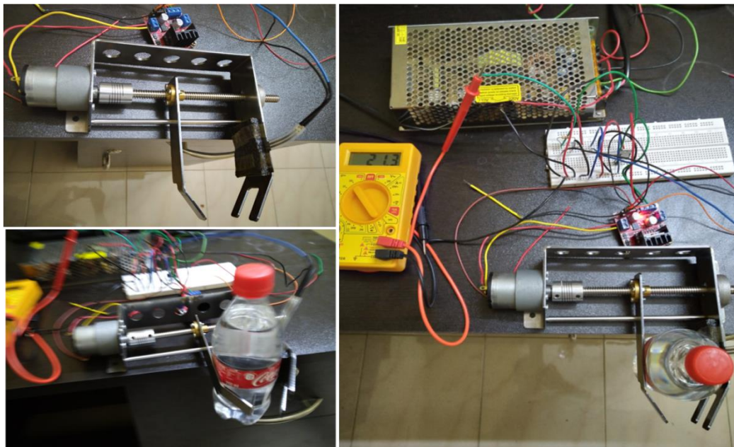
Figure 10. L.S.Gripper assembly operation
