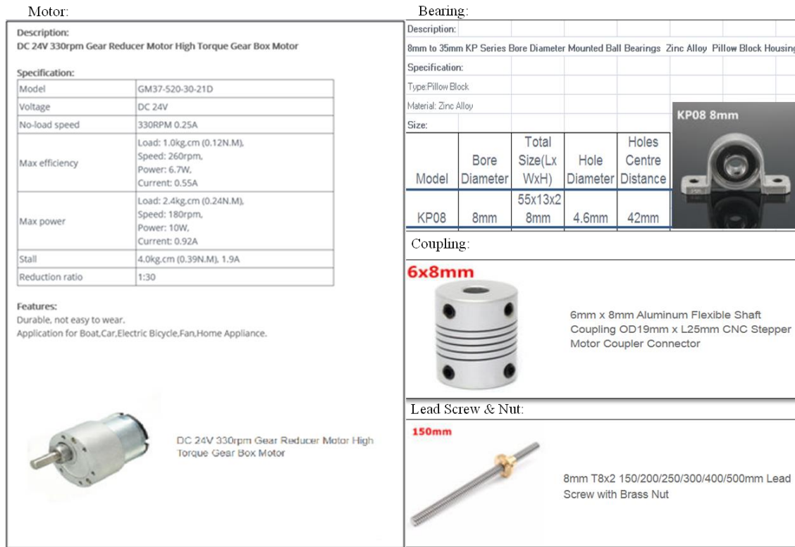
Figure 3. Component selection & specification
