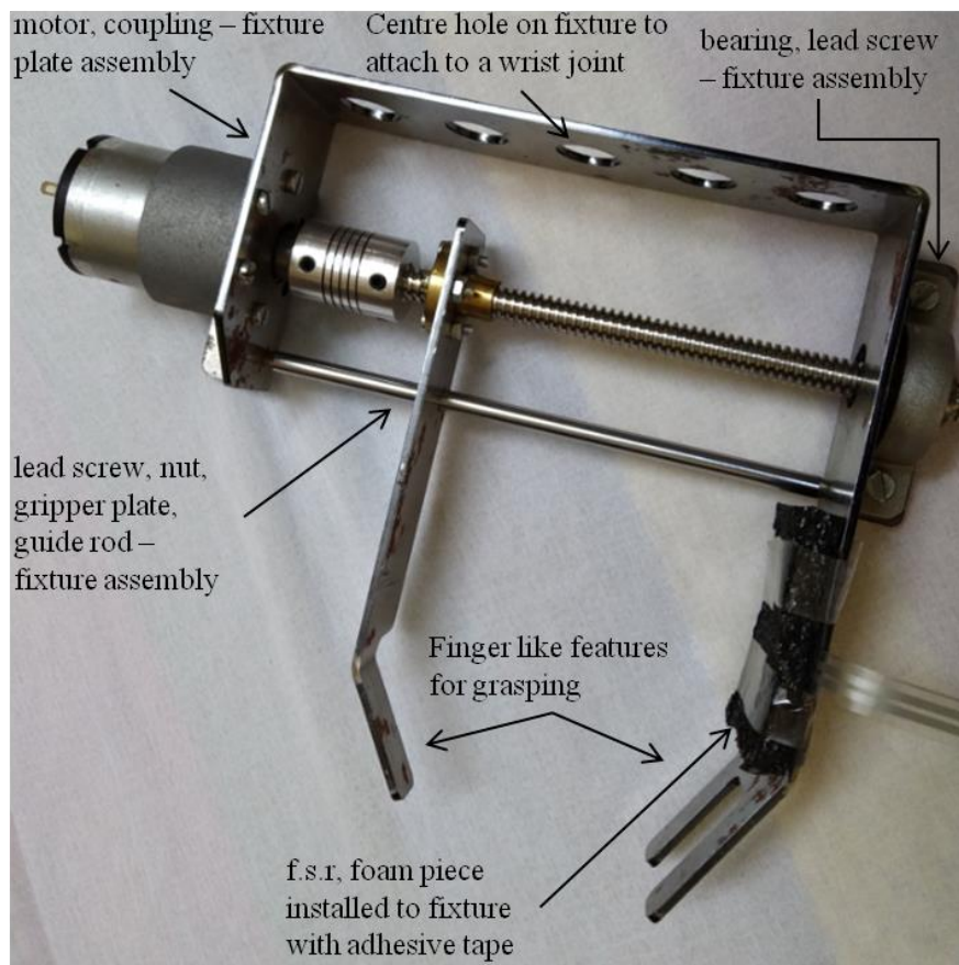
Figure 9. L.S.Gripper assembly construction
