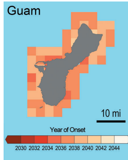
Figure 13. Projected year of onset of annual severe bleaching caused by ocean warming for corals in the waters of Guam. Under projected warming, coral reefs will experience annual bleaching beginning in about 2035 in the Mariana Archipelago. Source: Adapted from Keener et al. 2018, using data from van Hooidonk et al. 2016.
