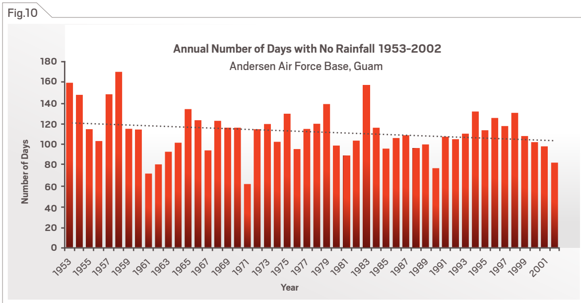
Figure 10. Annual number of days with no measurable rainfall at Andersen Air Force Base in Guam from 1953 to 2002. The black, dotted line shows no significant linear trend over time. Original figure by Abby Frazier, using data from the NOAA GHCN-Daily database (NOAA 2020c; Menne et al. 2012).
