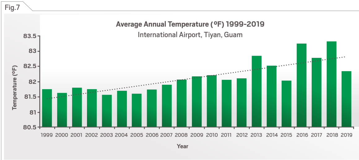
Figure 7. Average annual temperature at the International Airport in Tiyan, Guam, 1999–2019. The linear trend (black, dotted line) shows an increase over time. Original figure by Abby Frazier, using data from the NOAA GHCN-Daily database (NOAA 2020c; Menne et al. 2012).
