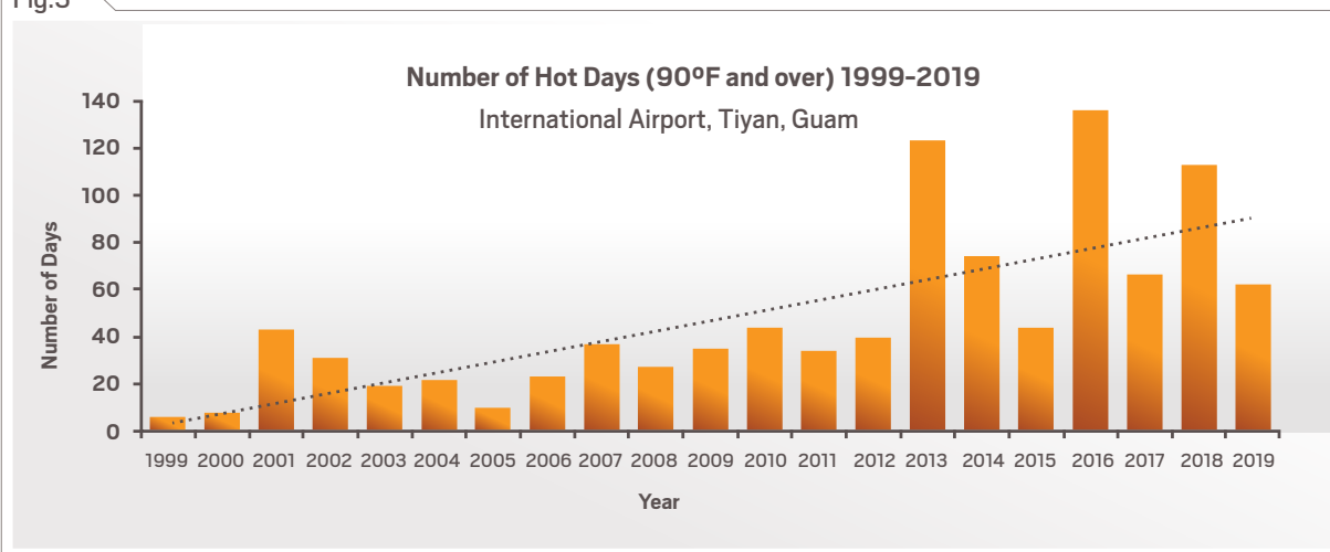
Figure 3. Annual number of days with maximum temperature 90°F (32°C) or hotter (at or above the 95th percentile of the data record) at the International Airport in Tiyan, Guam, from 1999 to 2019. The trendline (black, dotted line) shows there has been an increase in the annual number of hot days during this recent 21-year period. It should be noted that this station experienced equipment malfunctions from 2013 to 2019 that may have affected the maximum temperature readings. Original figure by Abby Frazier, using data from the NOAA GHCN-Daily database for 1999–2019 (NOAA 2020c; Menne et al. 2012).
