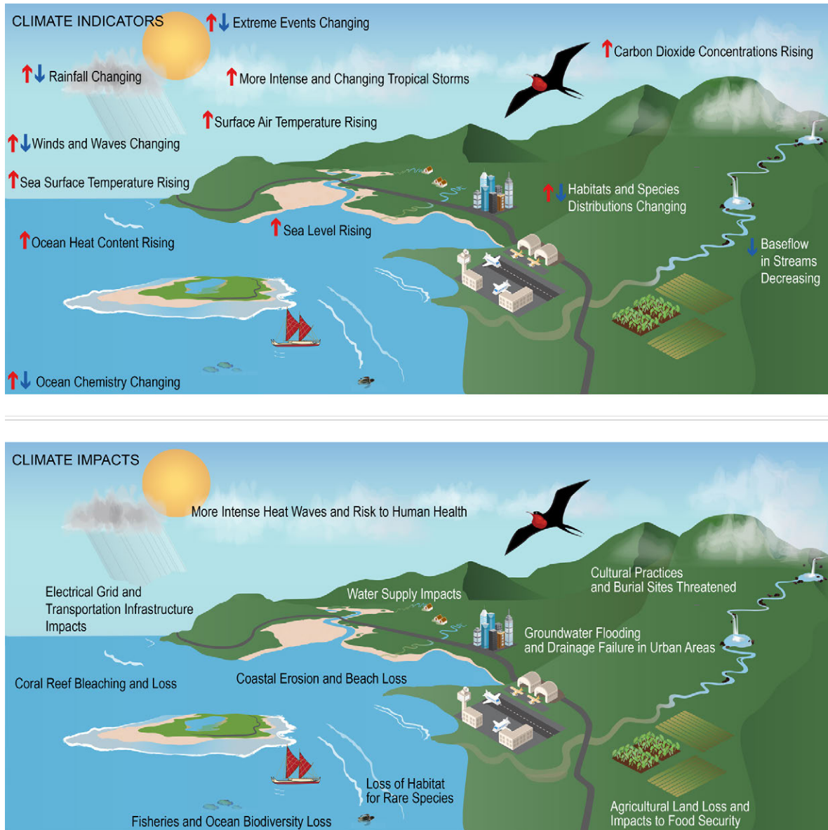
Figure 1. Observed changes in key climate indicators (top) in the Pacific Islands, such as carbon dioxide concentrations, sea surface temperatures, and species distributions result in impacts (bottom) to multiple sectors and communities, including built infrastructure, natural ecosystems, and human health. In the top panel, red arrows signify an indicator is increasing, while blue arrows show the indicator is decreasing. A red and blue arrow appear together for an indicator that is changing and the direction of change varies. Source: From Keener et al. 2018.
