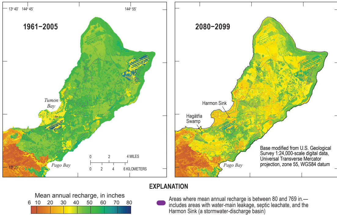
Figure 15. The distribution of average annual groundwater recharge (in inches) estimated for the Northern Guam Lens Aquifer for historic (1961–2005, left) and future (2080–2099, right) climate conditions. Source: Gingerich et al. 2019c.
