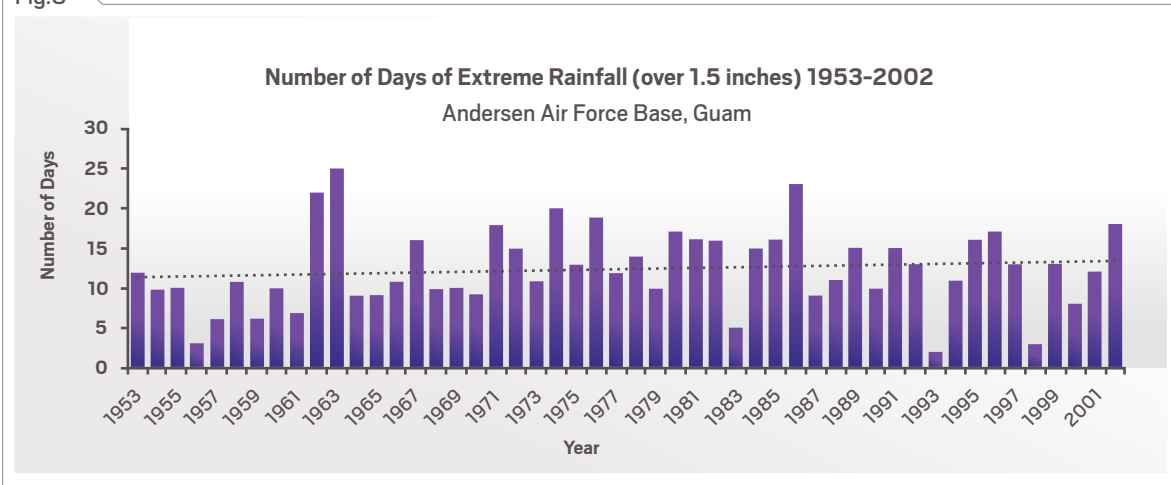
Figure 8. Annual number of extreme rainfall days, or days with daily rainfall totals exceeding the 95th percentile (approximately 1.5 inches) of the distribution at Andersen Air Force Base, Guam, from 1953 to 2002. The linear trend (black, dotted line) shows no trend over time. Original figure by Abby Frazier, using data from the NOAA GHCN-Daily database (NOAA 2020c; Menne et al. 2012).
