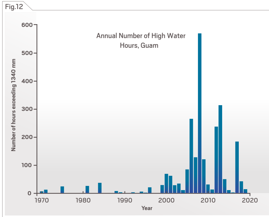
Figure 12. The number of high water hours per year at Guam’s coast, 1970 to 2019. The high-water threshold (1340 mm, 4.4 feet) is defined as the Mean Higher High Water level plus 1/3 of the difference between that and the Mean Lower Low Water level at the tide gauge (that is, water levels above the daily average highest tide plus a factor of the typical tidal amplitude). High water hours per year are affected by seasonal factors (such as monsoon activity), cyclical phenomenon (such as ENSO and Pacific Decadal Oscillation), and sea level rise. Source: Figure courtesy of Matthew Widlansky, with data from the University of Hawai’i Sea Level Center Station Explorer ( https://uhslc.soest.hawaii.edu/stations/?stn=053#datums ).
