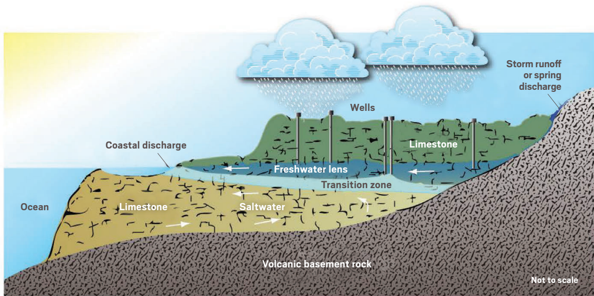
Figure 14. Schematic cross-section of the Northern Guam Lens Aquifer. Source: Adapted from Gingerich and Jensen 2010.
