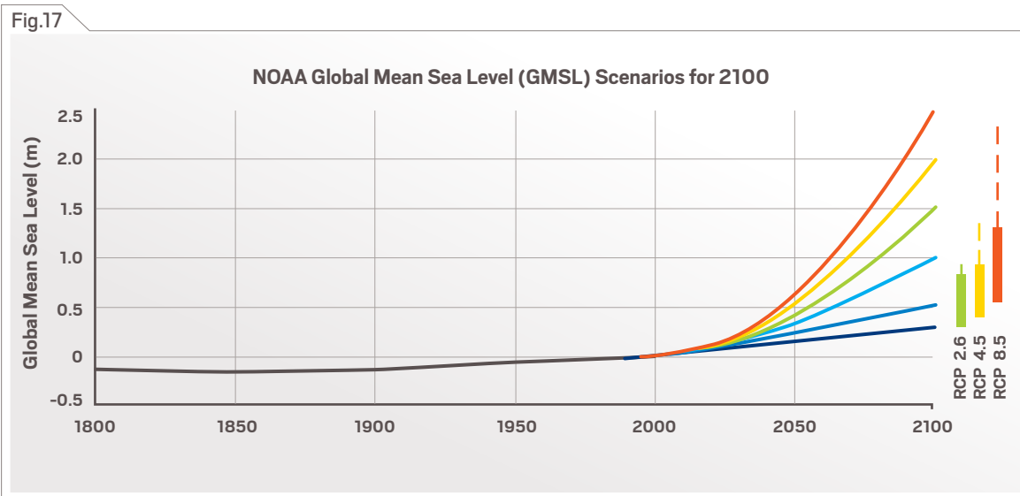
Figure 17. Six representative Global Mean Sea Level (GMSL) rise scenarios for 2100 (6 colored lines) relative to historical geological, tide gauge and satellite altimeter GMSL reconstructions from 1800–2015. The colored boxes show central 90% conditional probability ranges of RCP-based GMSL projections from recent studies. Dashed lines extending from the boxes show the median contribution from Antarctic melt from recent studies. Source: Sweet et al. 2017.
