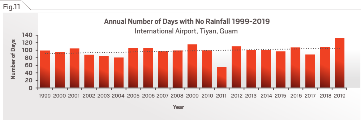
Figure 11. Annual number of days with no measurable rainfall at the International Airport in Tiyán, Guam, from 1999 to 2019. The linear trend (black, dotted line) shows no significant trend over time. Original figure by Abby Frazier, using data from the NOAA GHCN-Daily database (NOAA 2020c; Menne et al. 2012).
