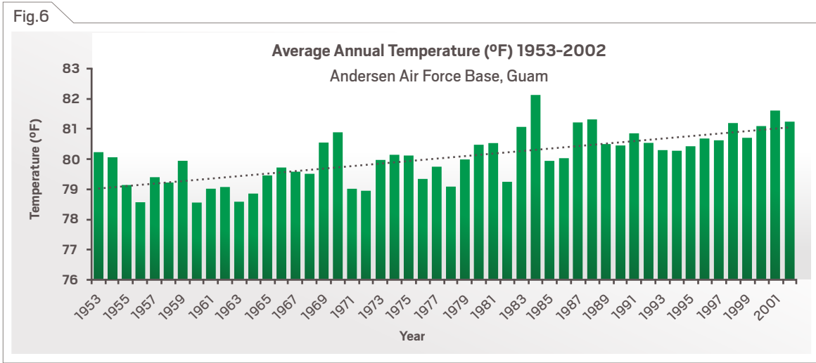
Figure 6. Average annual temperature at Andersen Air Force Base in Guam 1953–2002. The long-term linear trend indicated by the black, dotted line shows an increase over time. Original figure by Abby Frazier, using data from the NOAA GHCN-Daily database (NOAA 2020c; Menne et al. 2012).
