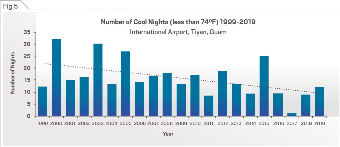
Figure 5. Annual number of nights with minimum temperature less than 74°F (23.3°C)—the 10th percentile of the data record—at the International Airport in Tiyan, Guam, from 1999 to 2019. The trendline (black, dotted line) shows a decrease in frequency of cool nights over the recent 21-year period. Original figure by Abby Frazier, using data from the NOAA GHCN-Daily database (NOAA 2020c; Menne et al. 2012).
