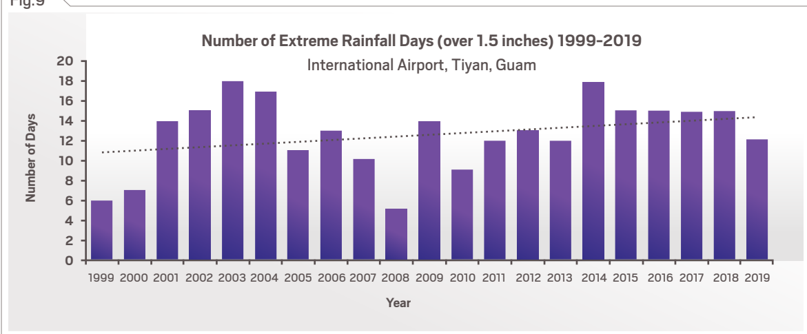
Figure 9. Annual number of extreme rainfall days, or days with daily rainfall totals exceeding the 95th percentile (approximately 1.5 inches) of the distribution at the International Airport in Tiyan, Guam, from 1999 to 2019. The linear trend (black, dotted line) shows no significant trend over time. Original figure by Abby Frazier, using data from the NOAA GHCN-Daily database (NOAA 2020c; Menne et al. 2012).
