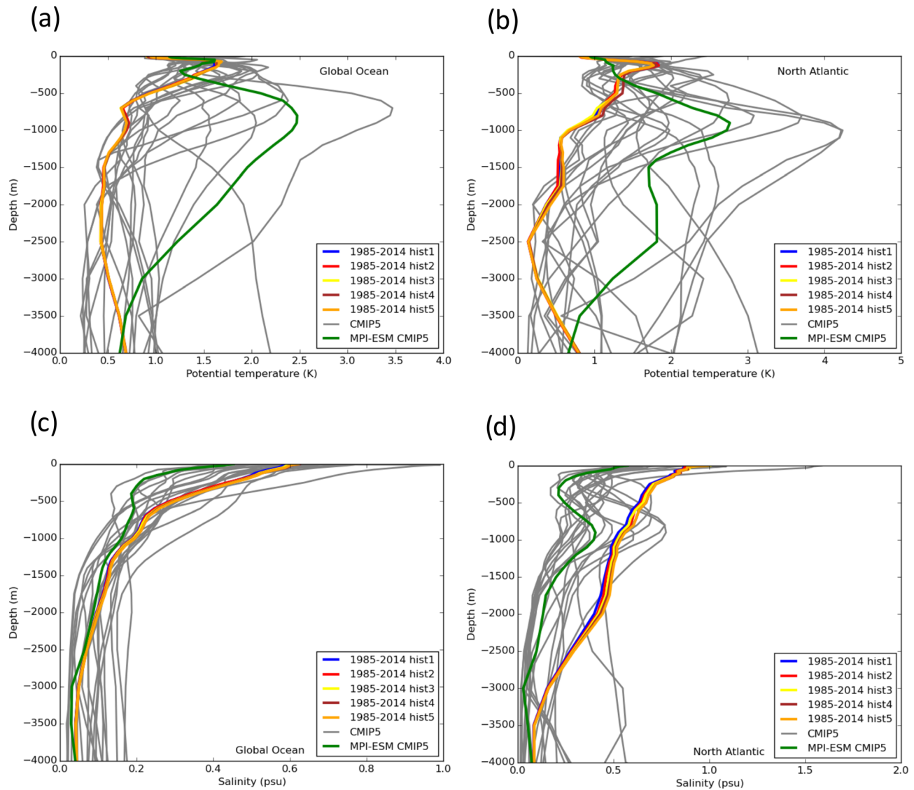
Figure 9. Profiles of mean absolute error calculated from each grid point for the (a) global ocean and (b) North Atlantic Ocean potential temperature ( ^{\circ}\text{C} ) for DJF 1985–2014 of the five ensemble members of the historical AWI-CM simulation (in colors) and for DJF 1976–2005 of CMIP5 simulations (in gray, each line representing one CMIP5 model, green representing the MPI-ESM CMIP5 model). Panels (c) and (d) as (a) and (b) but for salinity (psu). The reference climatology is the Polar Science Center Hydrographic Climatology (PHC, updated from Steele et al., 2001).
