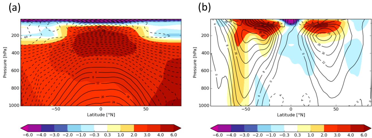
Figure 18. (a) Zonal mean temperature response ( ^{\circ}\text{C} ), (b) zonal mean zonal wind ( \text{m/s} ) response SSP370 scenario simulations (2071–2100, annual means) compared to historical simulations (1985–2014) (shaded contours). For both the scenario and the historical simulations, the five member ensemble means have been computed. The solid black lines represent positive values from the historical simulations and the dashed black lines negative values.
