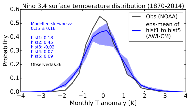
Figure 5. Probability distribution function (PDF) of sea surface temperature anomalies in the Niño 3.4 region for the historical period 1870–2014. The black line gives the observed Niño 3.4 PDF for the period 1870–2014 (Rayner et al., 2003), available for download from the National Oceanic and Atmospheric Administration (NOAA, https://www.esrl.noaa.gov/psd/gcos_wgsp/Timeseries/Nino34/ ). The ensemble-mean of the five historical members is given in blue; their range (min/max) is shaded in light blue.
