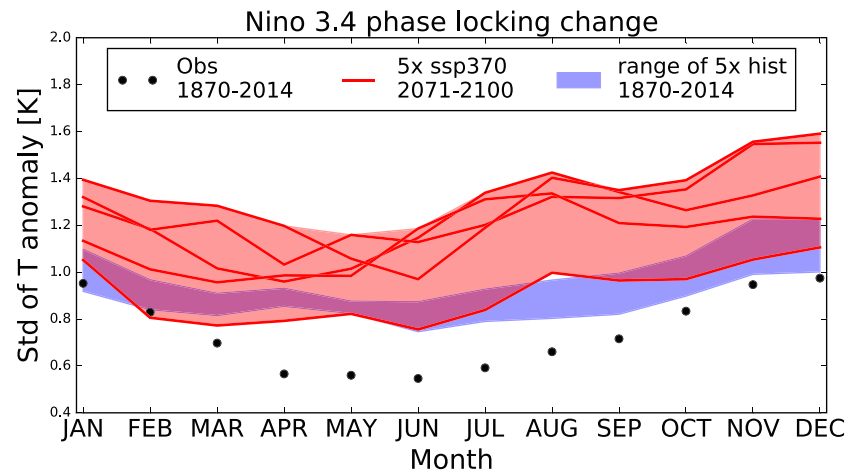
Figure 26. Seasonal phase locking of temperature anomalies in the Niño 3.4 region at the end of the 21st century (2071–2100) and for the period 1870–2014. Black dots give the monthly standard deviation of the observed Niño 3.4 index for 1870–2014 (Rayner et al., 2003). Red lines denote the standard deviations of the simulated Niño 3.4 indices for the five ssp370 ensemble members. The range of the model results is shaded in light blue (1870–2014, as in Figure 7) and in light red (2071–2100).
