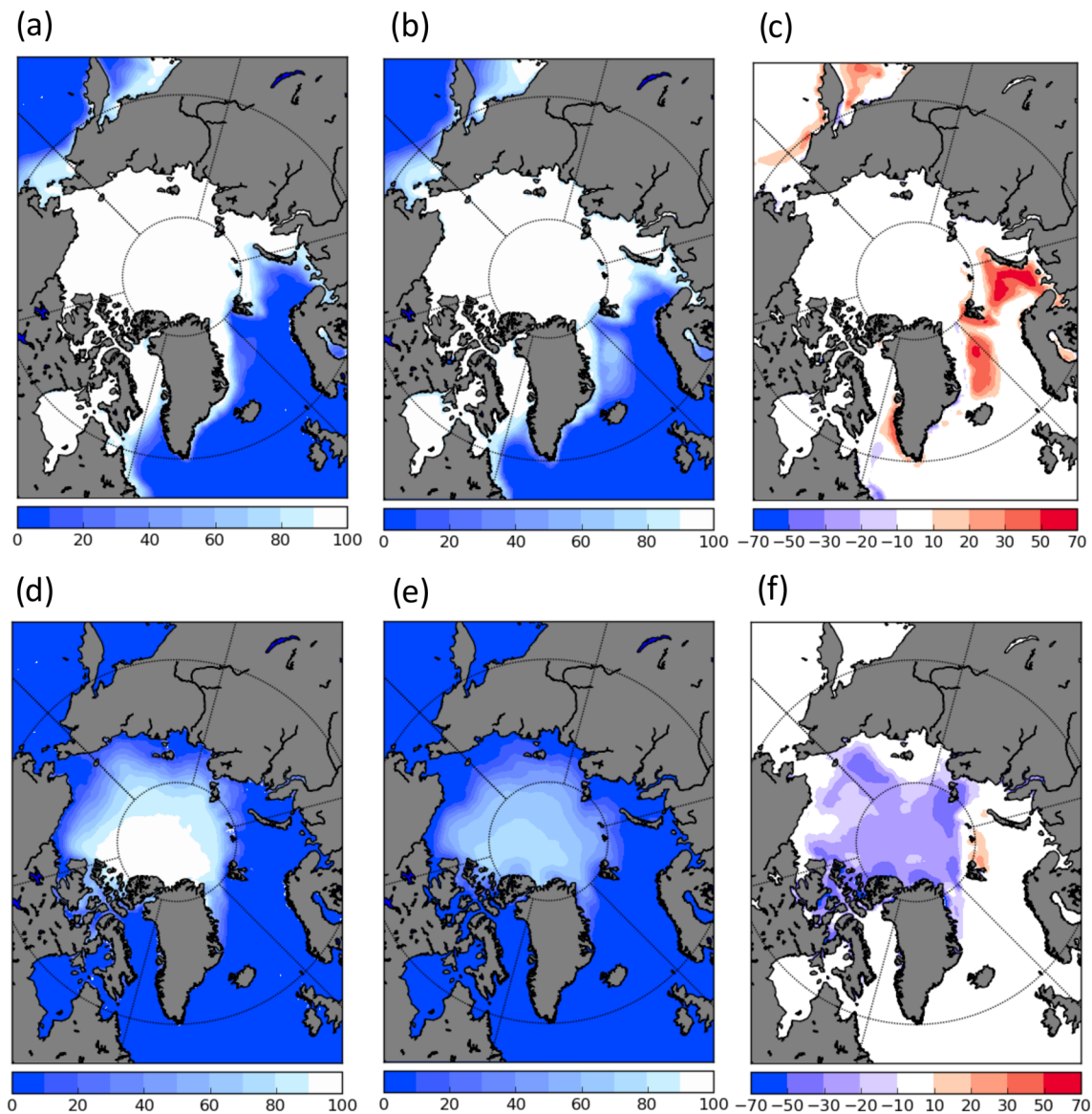
Figure 10. Arctic sea ice concentration (%) averaged over March 1985 to 2014 from (a) observations from the sea ice portal meereisportal.de (Grosfeld et al., 2016), (b) ensemble mean AWI-CM historical simulations, (c) ensemble mean AWI-CM historical simulation bias. Panels (d) to (f) same as (a) to (c) but for September 1985 to 2014.
