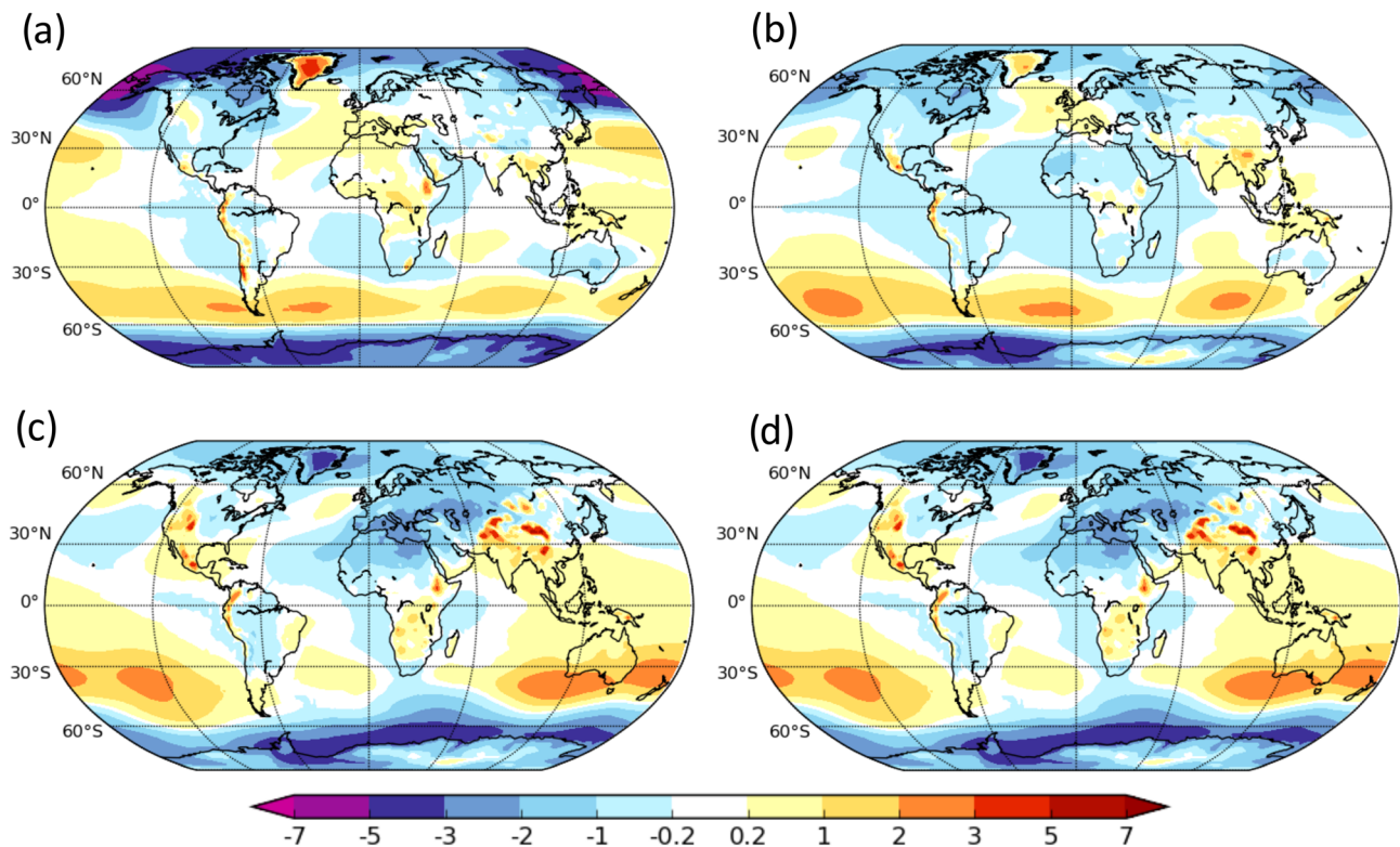
Figure 17. Mean sea level pressure (MSLP) response in SSP370 scenario simulations (2071–2100) compared to historical simulations (1985–2014). For both the scenario and the historical simulations, the five member ensemble means have been computed. (a) DJF, (b) MAM, (c) JJA, (d) SON.
