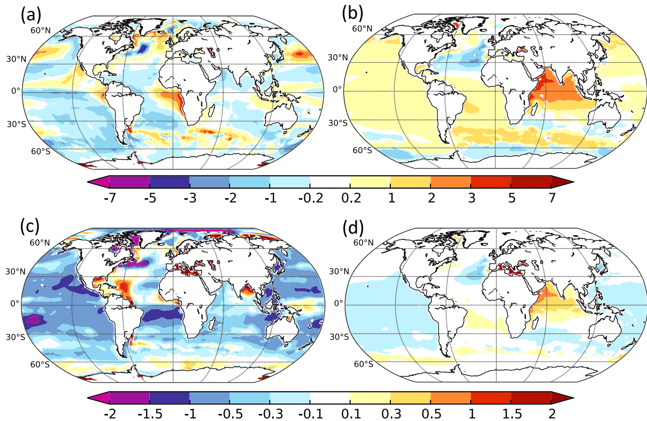
Figure 8. Bias of the annual mean potential temperature ( ^{\circ}\text{C} ) (a) at the surface, (b) at 1,000 m depth averaged over 1985–2014 of the first ensemble member of historical simulations compared to the Polar Science Center Hydrographic Climatology (PHC, updated from Steele et al., 2001). Panels (c) and (d) as (a) and (b) but for salinity (psu).
