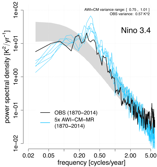
Figure 6. Power spectral densities (PSDs) of sea surface temperature anomalies in the Niño 3.4 region for the period 1870–2014. The black line gives the observed (OBS) spectrum after Rayner et al. (2003). The five historical ensemble members with AWI-CM are given in blue. Gray shading denotes the 5–95% confidence interval of an AR(1)-process fitted to OBS, based on a Monte Carlo approach with 10,000 realizations, as detailed by Rackow et al. (2018). The total (integrated) observed Niño 3.4 variance [ K^2 ] is 0.57; for AWI-CM-MR, the range is (0.75–1.01).
