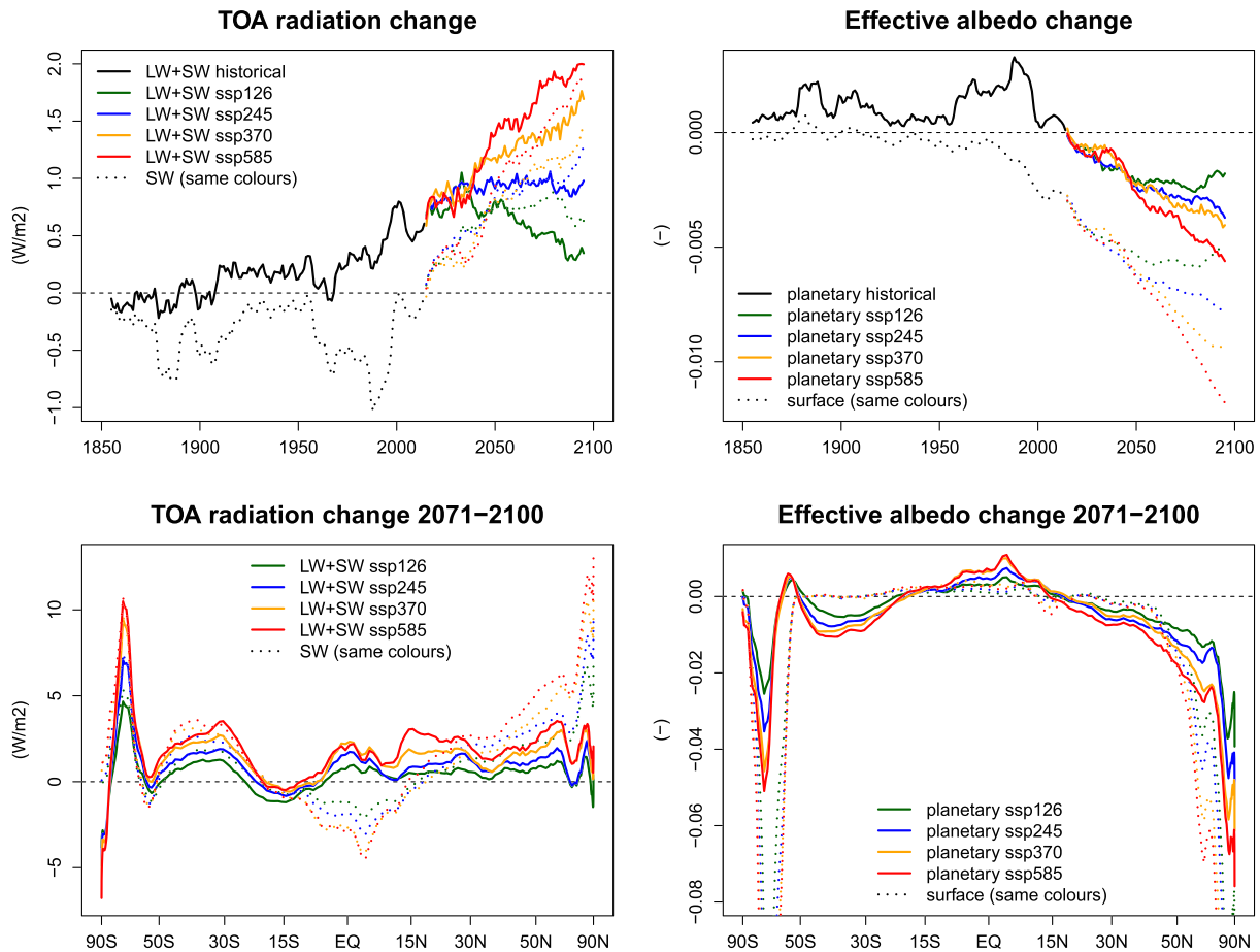
Figure 23. Annual-mean changes in the energy budget, relative to piControl (delta approach). (a) Top of atmosphere (TOA) net total (longwave (LW) + shortwave (SW); solid) and net shortwave (dashed) radiation time series after application of an 11-year running-mean, for the historical (black) and scenario (colors) simulations. Positive is downward. (b) Changes in the effective albedo diagnosed as upwelling divided by downwelling shortwave radiation at the TOA (planetary; solid) and at the surface (dashed). Panels (c) and (d) same as (a) and (b) but as zonal means averaged over the period 2071–2100 (scenario simulations only), plotted against \sin(\text{latitude}) to reflect equal-area global contributions. Extreme negative values of effective surface albedo changes, reaching about -20\% in both polar regions, are truncated in (d) to increase the visibility of changes in lower latitudes. Only the respective first ensemble member of the historical and SSP370 scenario simulations is shown.
