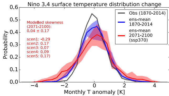
Figure 24. Change of the probability distribution function of sea surface temperature anomalies in the Niño 3.4 region for 2071–2100 (red line). Compared to 1870–2014 (black and blue lines), extreme anomalies become more likely while the probability of low to medium anomalies decreases. The range of the model results is shaded. ENSO asymmetry (positive skewness) decreases compared to 1870–2014 (see Figure 5). All data have been linearly detrended, and the seasonal cycle has been removed.
