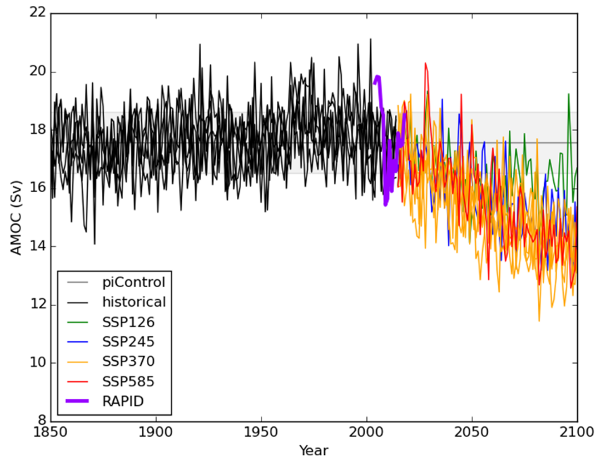
Figure 20. Maximum Atlantic meridional overturning circulation (AMOC) (Sv) at 26°N for piControl, historical, scenario simulations, and from RAPID observations (Smeed et al., 2019). For piControl, the mean value is indicated by the straight gray line and the standard deviation over the 500 year period is shown by the gray shaded area. Values of individual years are not shown for piControl.
