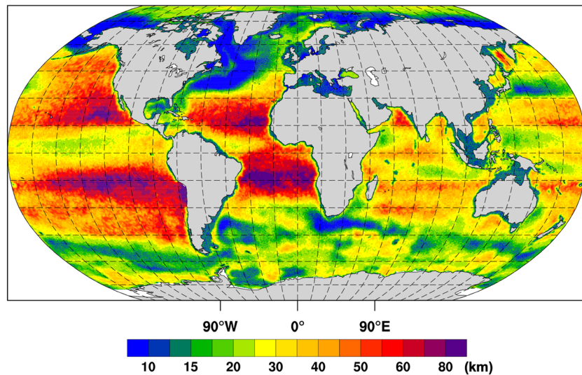
Figure 1. Spatial resolution (in km) of the FESOM MR grid used in AWI-CM-1-1-MR for the CMIP6 DECK and ScenarioMIP simulations. Resolution is locally increased up to 8 km in regions of high sea surface height (SSH) variability as observed by satellites.
