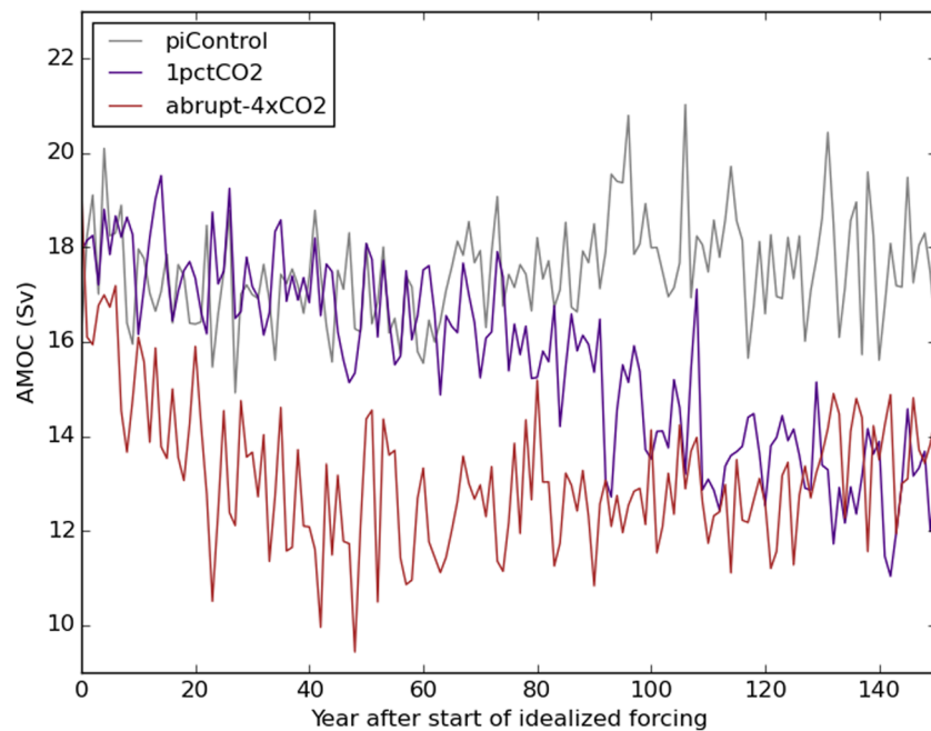
Figure 21. Maximum Atlantic meridional overturning circulation (AMOC) at 26°N (Sv) for piControl and the idealized simulations 1pctCO 2 and abrupt-4xCO 2 . Please note that the branch-off point for both idealized simulations is Year 250 of piControl simulation. The year on the x-axis represents the year after this branch-off point and therefore the year after the start of the idealized forcing.
