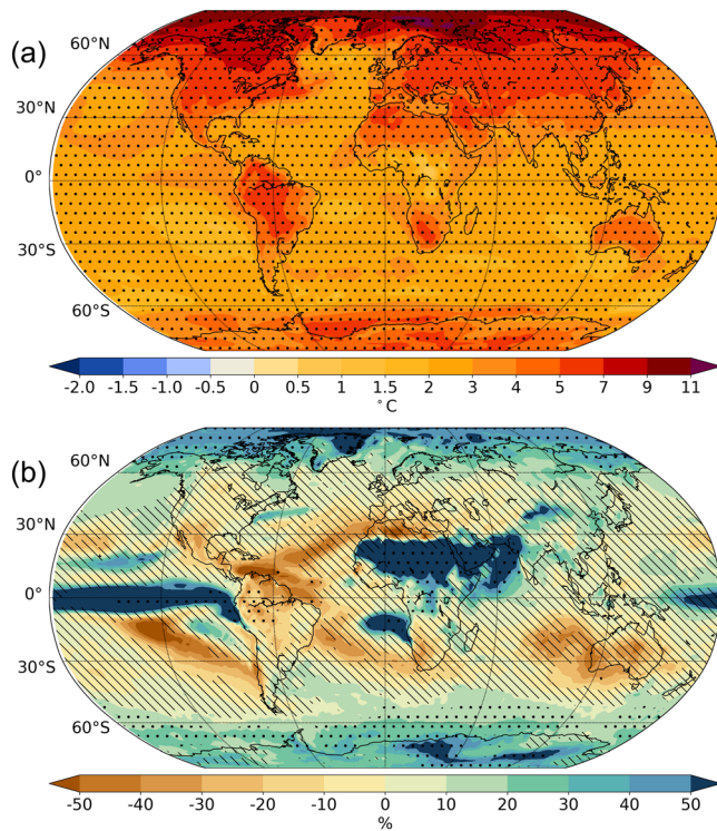
Figure 14. (a) Annual mean 2 m temperature and (b) precipitation response according to the SSP585 scenario 2071–2100 compared to the historical period 1985–2014. Dotted (hatched) areas represent areas where simulated changes are larger than (smaller than) 2 standard deviations (1 standard deviation) of the internal variability based on yearly means of the 500-year control simulation.
