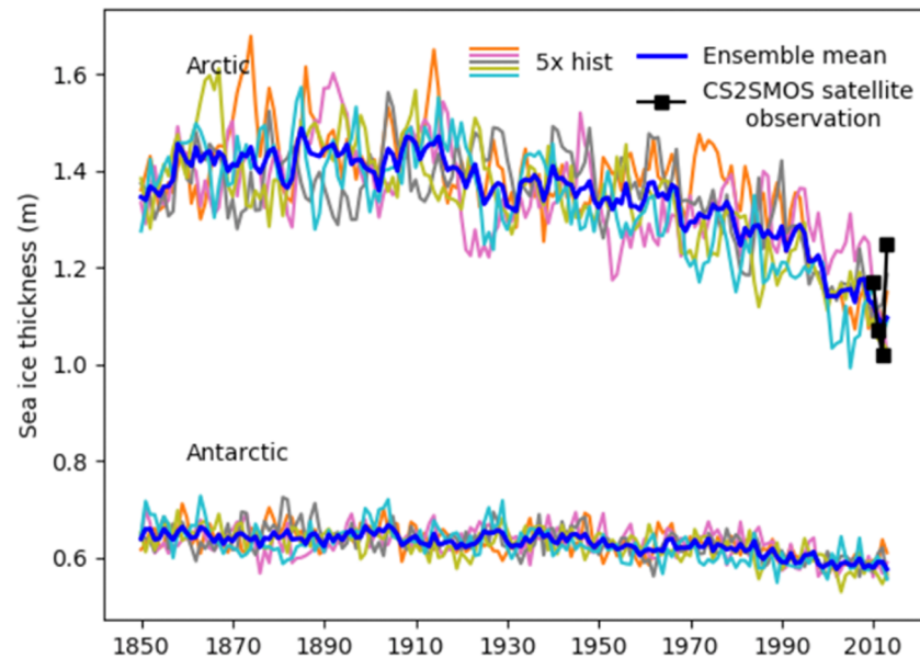
Figure 16. Sea ice thickness in the historical simulation during the frozen season in the Arctic (averaged over December to March for each year) and the Antarctic (averaged over May to September for each year). The blue lines show the ensemble mean of the five members indicated by different colors. Satellite estimates for the Arctic from merged CryoSat-2 and SMOS data (CS2SMOS product) are shown by black squares.
