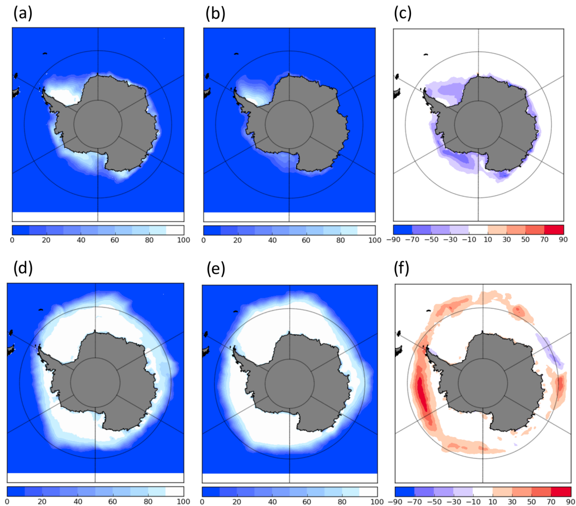
Figure 11. (a–f) Same as Figure 10 but for Antarctica.
