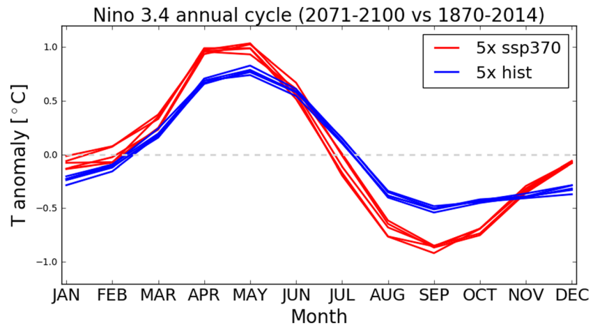
Figure 25. The annual cycle within the Niño 3.4 box for historical (1870–2014) and future (2071–2100) conditions. Five ensemble members each are shown for the historical simulations (blue) and the ssp370 scenario (red). The different annual means (historical: 25.4°C, scenario: 28°C) have been removed to highlight the different characteristics of the annual cycles.
