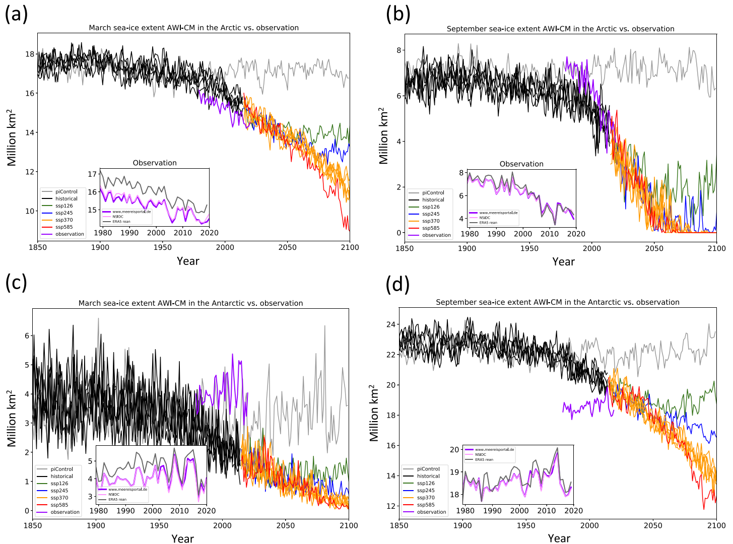
Figure 15. (a) March and (b) September sea-ice extent in the Arctic (million km 2 ). Panels (c) and (d) same as (a) and (b) but for the Antarctic region. The purple line indicates the observed sea-ice extent from the sea ice portal meereisportal.de (Grosfeld et al., 2016). For comparison, observational National Snow and Ice Data Center (NSIDC) (Fetterer et al., 2017) and ERA5 reanalysis (Copernicus Climate Change Service [C3S], 2017; Hersbach et al., 2020) sea-ice extent are shown in inlays along with the ones from sea ice portal. The observation uncertainty is small and does not affect the conclusions.
