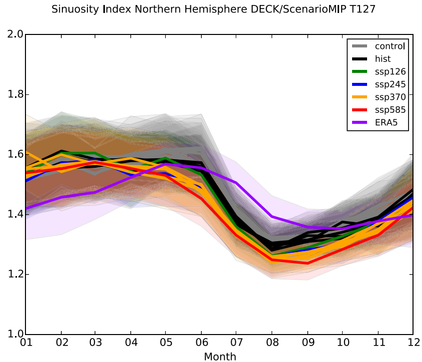
Figure 19. Monthly sinuosity index (unity) in the Northern Hemisphere according to Cattiaux et al. (2016) from control, historical, scenario simulations, and from ERA5 reanalysis data (Copernicus Climate Change Service [C3S], 2017; Hersbach et al., 2020). Historical and scenario simulations are taken for the 30-year periods 1985–2014 and 2071–2100, respectively. From the control simulation, all 30-year periods corresponding to the different ensemble members of historical and scenario simulations are considered resulting in multiple curves. The shaded areas represent the standard deviations of the 30 monthly sinuosity values for each simulation.
