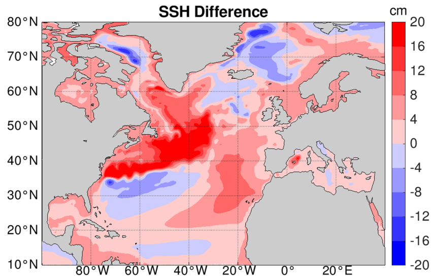
Figure 22. Difference of the sea surface height (SSH) between the mean over 2071–2100 (SPP370) and the mean over 1985–2014 (historical run) averaged over five ensemble members. Only the dynamical sea level part is shown (i.e., contributions from thermal expansion and water mass changes are not considered).
