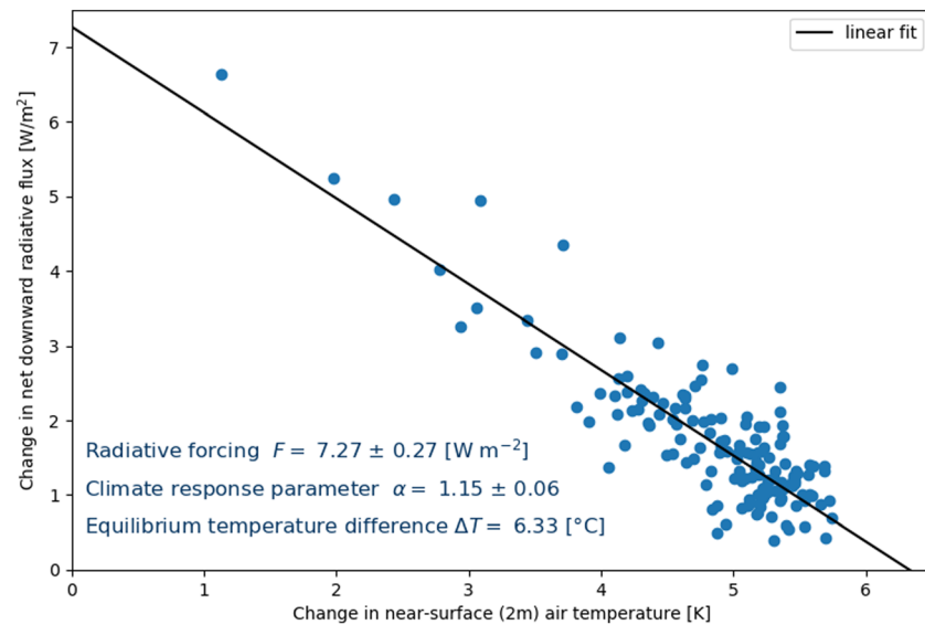
Figure 12. Gregory plot (Gregory et al., 2004) from the abrupt-4xCO 2 compared to the piControl simulation. For each year, the near-surface (2 m) air temperature change between abrupt-4xCO 2 and piControl simulation is plotted against the change in net downward radiative flux between the two simulations. The more the abrupt-4xCO 2 simulation approaches the equilibrium, the smaller the difference in net downward radiative flux compared to the reference simulation becomes. To compute the initial radiative forcing, a regression is built from all data points and extrapolated to a change in near-surface air temperature of 0°C. \alpha is the climate response parameter, indicating the strength of the climate system's net feedback (radiative feedback divided by temperature response). To compute the equilibrium temperature difference, the regression is extrapolated to the equilibrium (difference in net shortwave radiation = 0).
