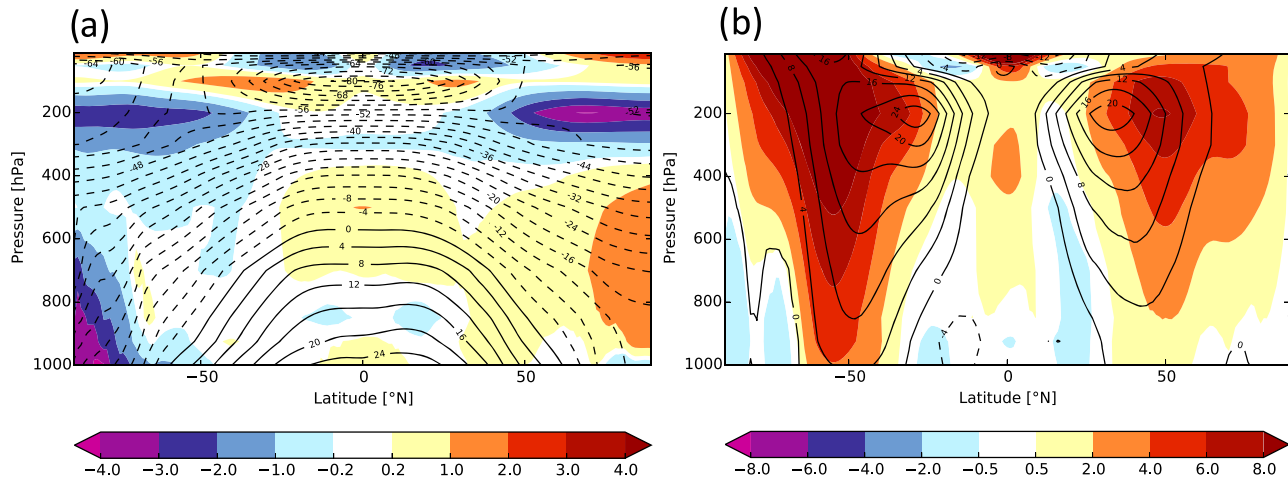
Figure 4. (a) Annual mean zonal mean temperature (°C) and (b) annual mean zonal mean zonal wind (m/s) as an ensemble mean over the five historical realizations for 1985–2014 compared to ERA5 climatology (Copernicus Climate Change Service [C3S], 2017; Hersbach et al., 2020) from 1985 to 2014. Solid lines represent temperatures at or above 0°C and westerly zonal wind speeds from the ERA5 climatology, dashed lines represent temperatures below 0°C and easterly wind speeds, and contours represent biases.
