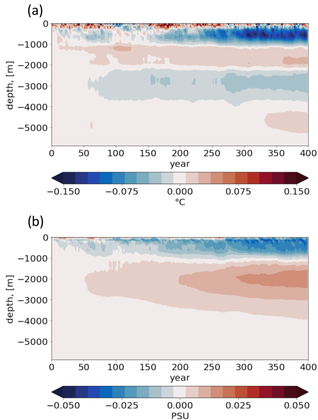
Figure 2. Vertical profiles of globally averaged (a) ocean temperature and (b) salinity in the last 400 years of the 500 years of piControl simulation (relative to the beginning of this 400 year time period). The last 400 years cover all simulations branched off since the first branch-off point is in Year 150 of the piControl simulation, that is, 350 years before the end of the piControl simulation (see Table 1).
