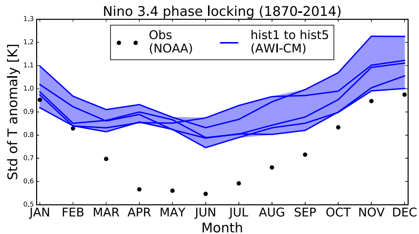
Figure 7. Seasonal phase locking of sea surface temperature anomalies in the Niño 3.4 region for 1870–2014. Black dots give the monthly standard deviation of the observed Niño 3.4 index for 1870–2014 (Rayner et al., 2003); blue lines give the standard deviations of the simulated Niño 3.4 indices for each of the five historical ensemble members (hist1 to hist5). The range (min/max) spanned by the model results is shaded in light blue. All data have been linearly detrended and the seasonal cycle removed before computing the standard deviation.
