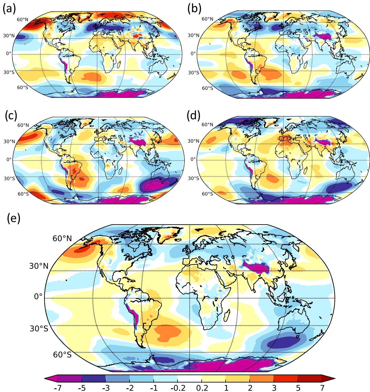
Figure 3. Mean sea level pressure (MSLP) bias (hPa) as an ensemble mean over the five historical realizations for 1985–2014 compared to ERA5 climatology (Copernicus Climate Change Service [C3S], 2017; Hersbach et al., 2020) from 1985 to 2014. (a) DJF, (b) MAM, (c) JJA, (d) SON, (e) annual mean.
