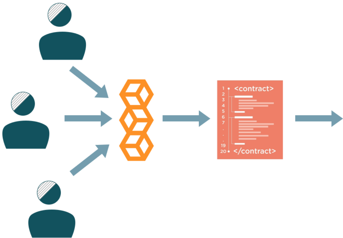
Figure 7: Privacy preserving patient data processing through smart contracts. Patient data is loaded into a blockchain, the subject data (of multiple subjects) sent to a smart contract ( Icon from here ). The smart contract is reviewed by an committee and/or public - it is assured that it will only release privacy preserving results, e.g. averages and/or time delayed results. Even if the data itself would reveal the subject's identity (whole genomes, faces, etc.)- the smart contract won't look at it. Potential in public health, life science research are humongous.
