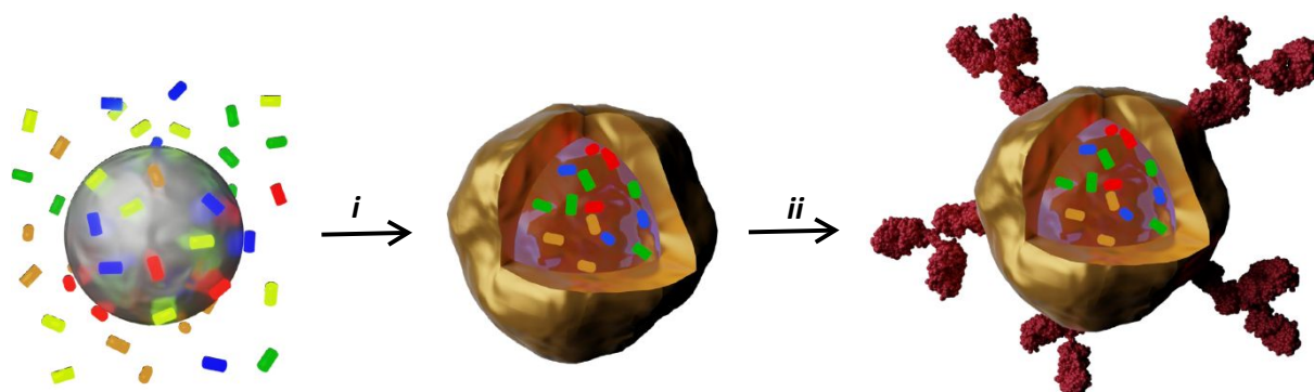
Scheme 1. Schematic representation of the synthesis of Raman reporter-encoded plasmonic nanocapsules through seed-mediated growth coupled to Galvanic replacement ( i ) and subsequent bioconjugation ( ii ).
