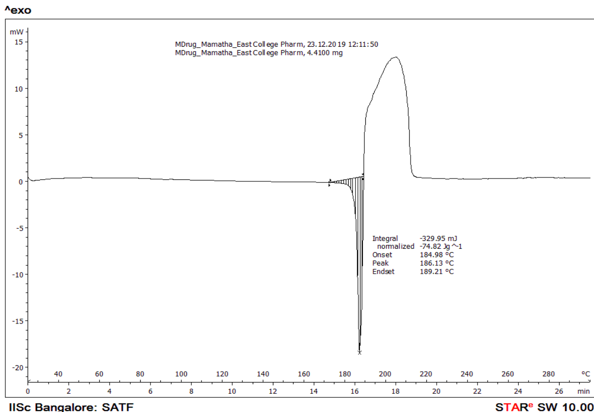
Figure 3: DSC Graph for Miconazole nitrate loaded SLN
