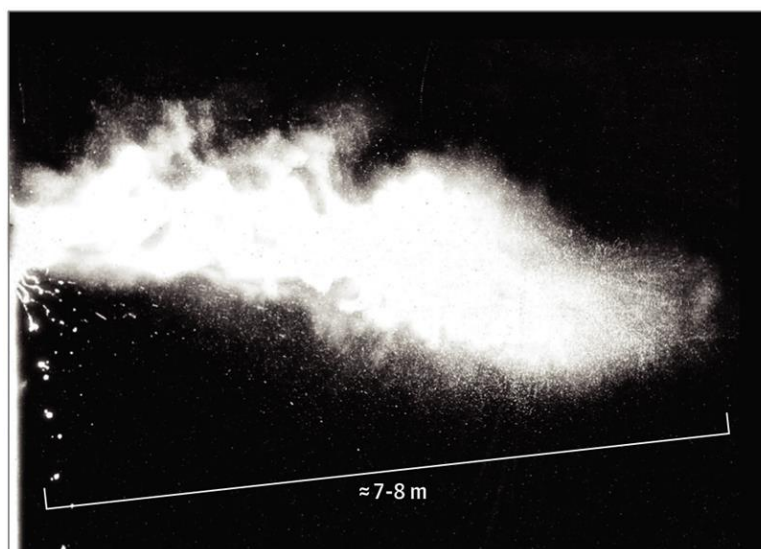
Figure 11 Multiphase Turbulent Gas Cloud From a Human Sneeze (from Bourouiba JAMA 2020)
