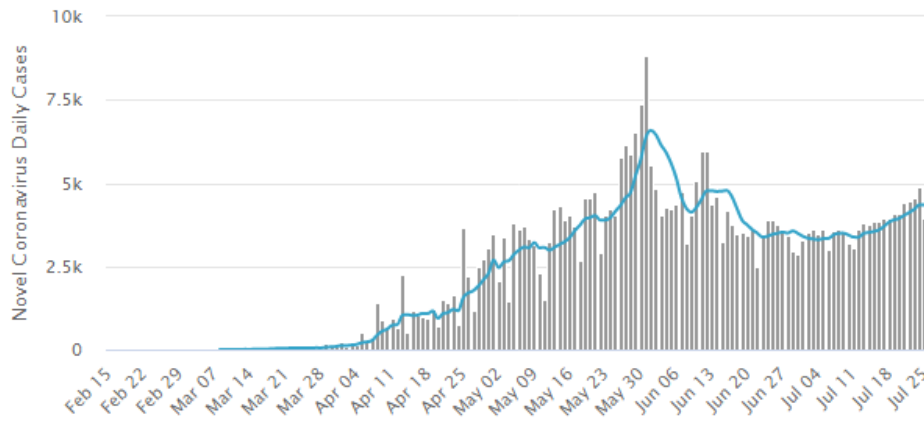
Daily New Cases. The blue line represents a 7-days moving average.
