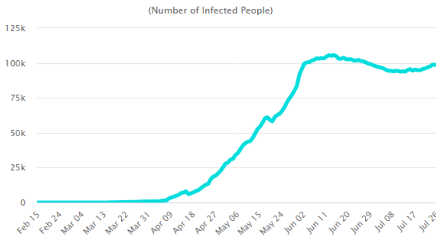
Number of infected people (active cases).
