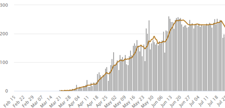
Daily victims ( www.worldometers.info/coronavirus ). Red line represents a 7-days moving average.
