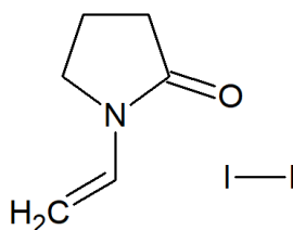
Figure 1. Chemical structure of povidone-iodine.
