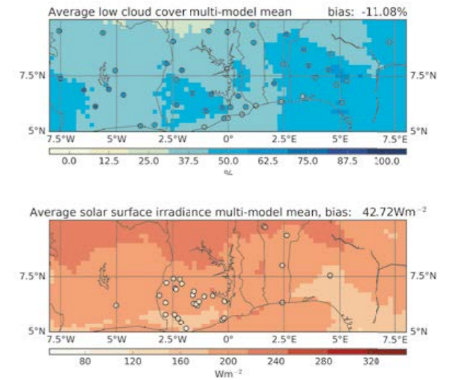
Figure 10. Average cloud cover (top) and surface solar irradiance (bottom) for the five NWP models (see Figure 9) used during the DACCWA field campaign period from 01 June to 31 July 2016. The coloured circles indicate corresponding station observations. Figure from Kniffka et al. [2020].
