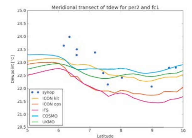
Figure 9. 2m-temperature (top) and dew point (bottom) along a meridional transect covering Benin, Togo and easternmost Ghana during 22 June – 31 July 2016. Dots are all available SYNOP stations, lines are zonal averages from five NWP models (ICON is run in two different configurations). Figure from Kniffka et al. [2020].
