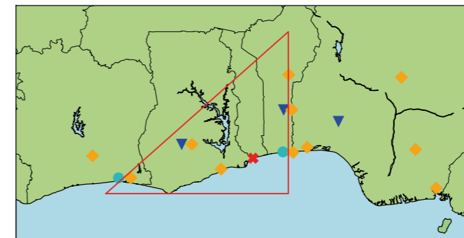
Figure 2. Location of measurement sites during the DACCIWA campaigns in 2016. Air Quality (AQ) sites measured the concentration of air pollutants. Supersites measured a range of meteorological and chemical parameters. Meteorological balloon sondes were released from eleven sites, partly in collaboration with West African weather services. Three research aircraft were based in Lomé (Togo) and sampled inside the red triangle. Evans et al. [2018]
