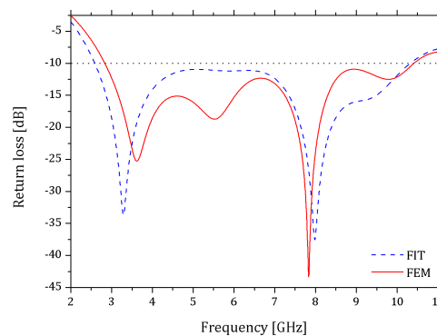
Figure 2. Return loss vs frequency calculated by FIT and FEM methods
