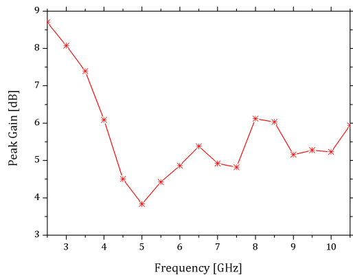
Figure 3. Peak gain of the proposed antenna vs frequency
