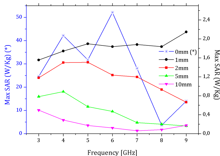
Figure 5. Numerical simulation SAR in the mammary tissue vs frequency at different distance between the UWB antenna and the breast. [(*) see left y-axis]
