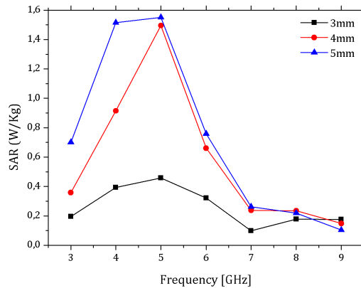
Figure 6. Numerical simulation SAR in the mammary tissue vs frequency by varying the size of the tumor
