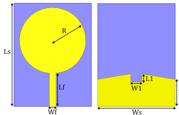
Figure 1. Geometry of the proposed antenna, left side: top view, right side: bottom view
