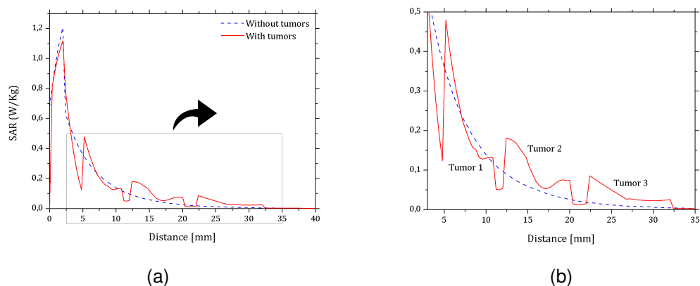
Figure 7. SAR distribution for 3 tumors at 3.62 GHz, (a) zoom out, (b) zoom in
