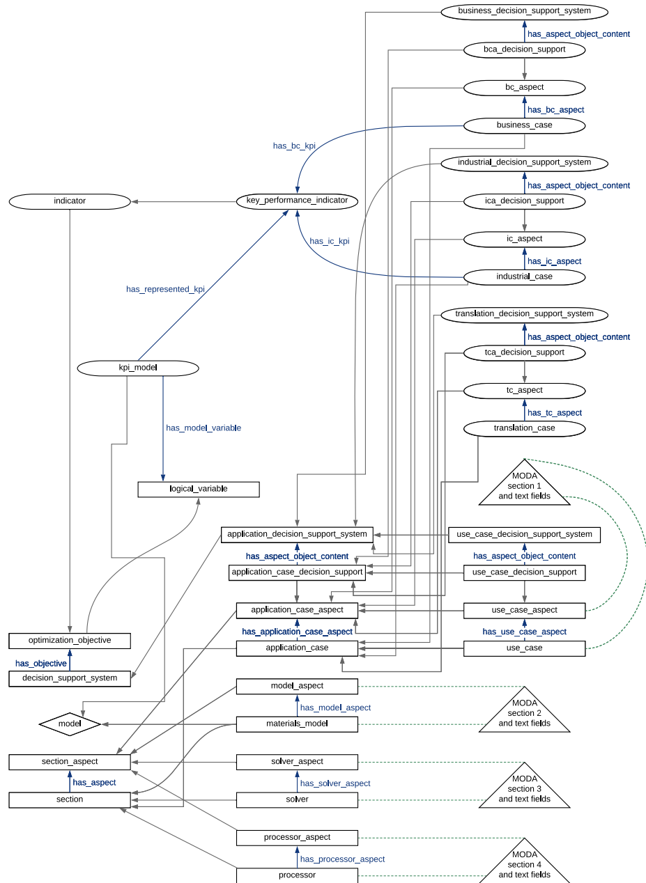
Fig. 1. Entities from MMTO version 1.3.4 (rounded boxes), OSMO version 1.6.6 (rectangular boxes), EMMO version 1.0.0 alpha 2 (diamond), MODA sections (triangles), and a subset of the relations defined by MMTO and OSMO, where grey arrows correspond to the transitive reduction of the rdfs:subClassOf relation, blue arrows to relations between individuals as indicated by arrow labels, and green dashed lines to correspondences between elements from MODA and OSMO.
