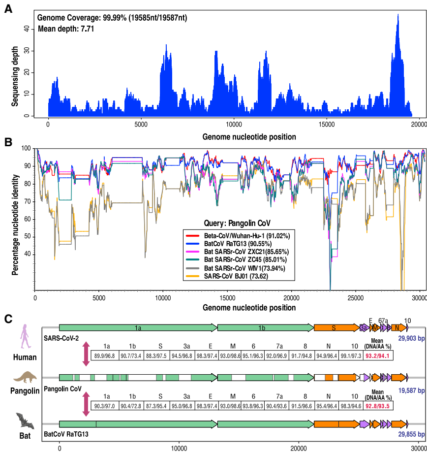
Figure 1. Genome-Related Analysis
