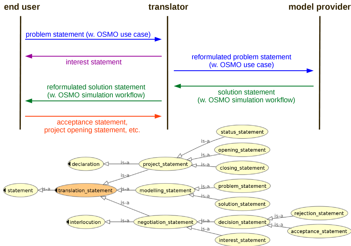
Figure 3.4. Top: Possible sequence of messages exchanged at a digital marketplace during negotiation of a materials modelling translation project [Hor20b]. Bottom: Class hierarchy for MMTO concepts related to exchange between potential partners during such interactions; the diagram was generated using the OWLViz protégé plugin; grey arrows labelled “is-a” denote subsumption ( \sqsubseteq ), i.e., rdfs:subClassOf .
