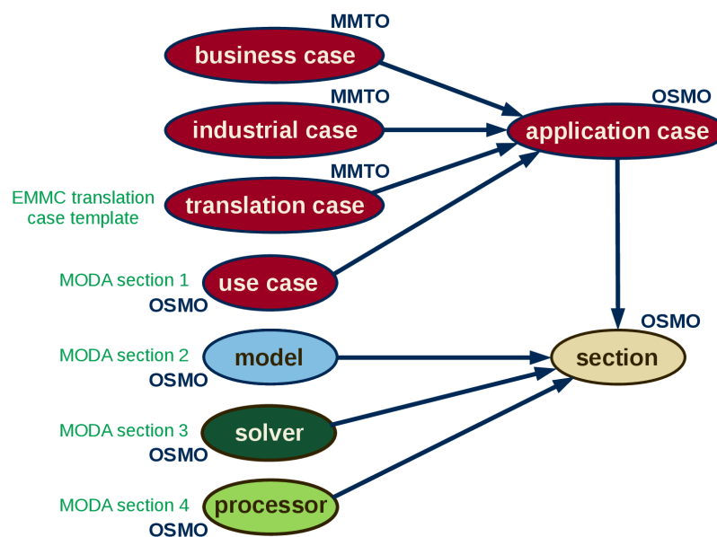
Figure 3.3. Section branch of MMTO and OSMO, cf. Section 3.3; arrows denote subsumption ( \sqsubseteq ).
