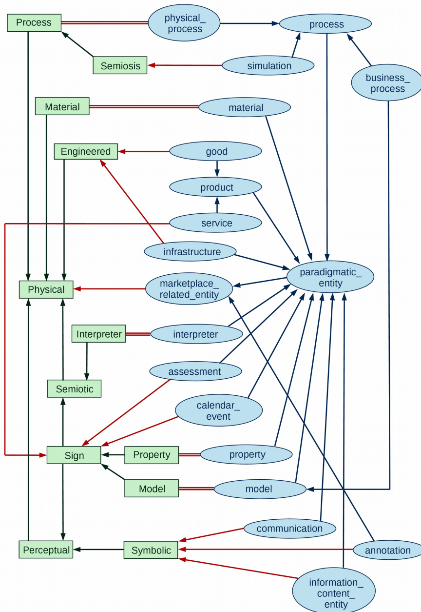
Figure 2.1. Fundamental categories, superclasses, and selected subclasses from the EVMPO (ellipses) together with related concepts from EMMO version 1.0.0 alpha 2 (rectangles); arrows between concepts denote subsumption, and double lines between concepts denote identity.
