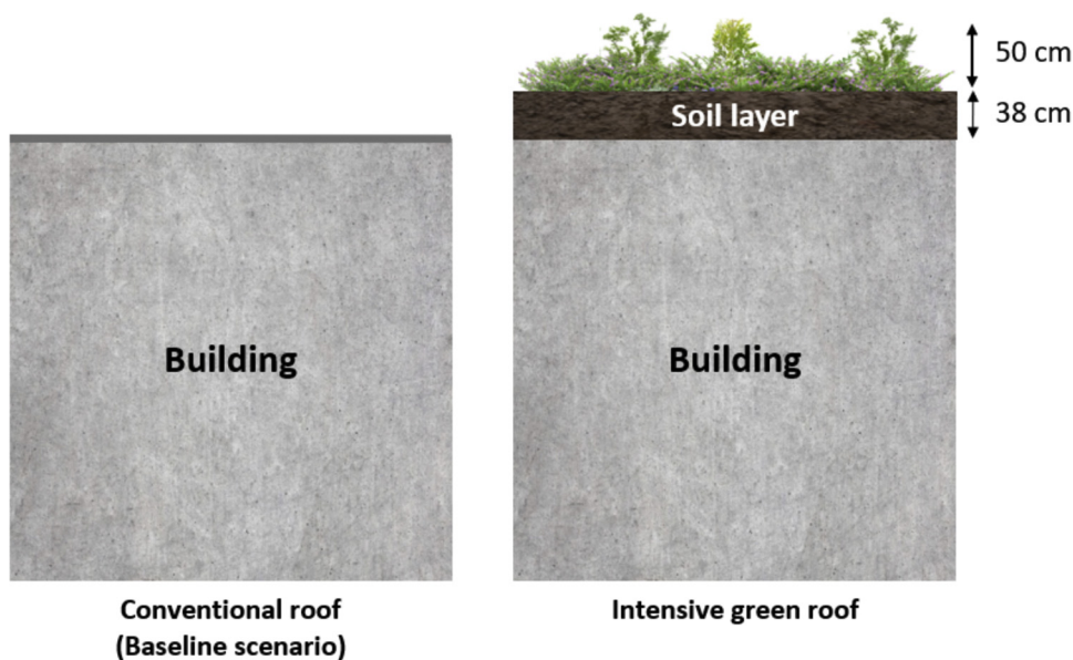
Fig. 4. Schematic illustration of the two different rooftop scenarios as specified in the customized ENVI-met greening data base.
