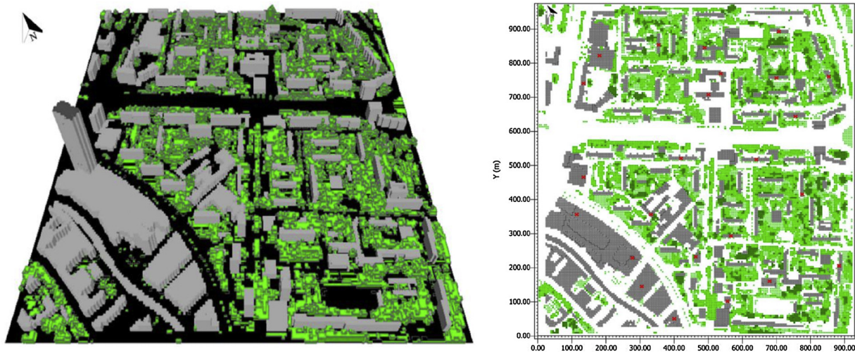
Fig. 3. Left: 3D-map of model area, colour coded by three main input layers: buildings (grey), vegetation (green) and asphalt surface (black). Right: 2-D map of study area input file. Red marks show locations of the 24 roof points that were used for PET computations. (For interpretation of the references to colour in this figure legend, the reader is referred to the web version of this article.)
