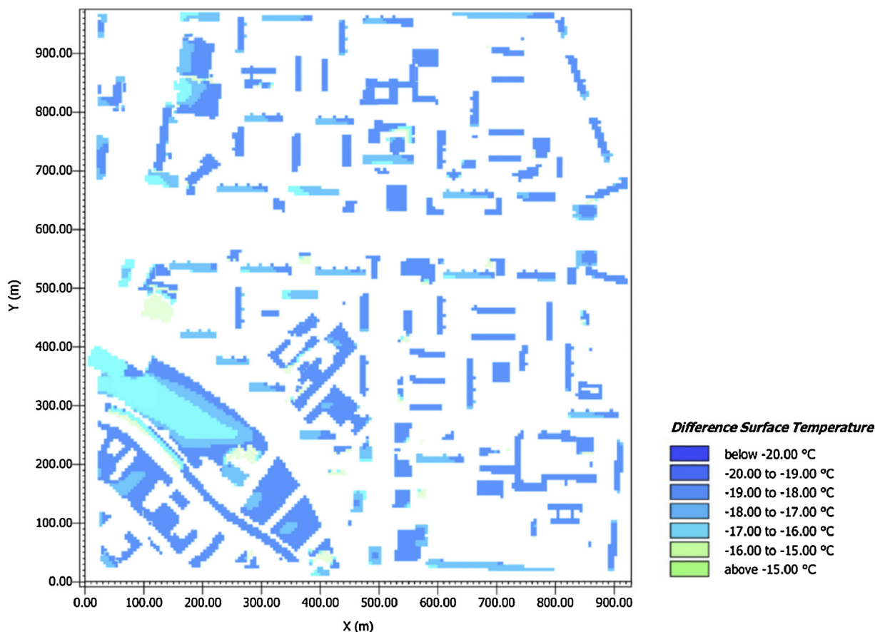
Fig. 6. Surface temperature difference between the intensive green roof scenario and the baseline scenario ( T_{s_{IGR}} - T_{s_{base}} ) at 14:00 CET for all roofs of the KMA area. (For interpretation of the references to colour in this figure legend, the reader is referred to the web version of this article.)
