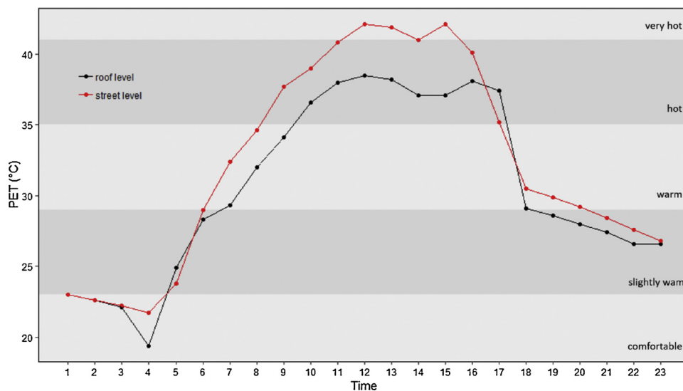
Fig. 7. Diurnal profile of the mean PET at the street level (red line) and roof level (black line) under the IGR scenario at 14:00 CET. Street-level values are averaged over the whole model domain whereas roof-level values are averaged over the 24 roof data points. Respective thermal perception of different PET ranges is indicated by grey shading. (For interpretation of the references to colour in this figure legend, the reader is referred to the web version of this article.)
