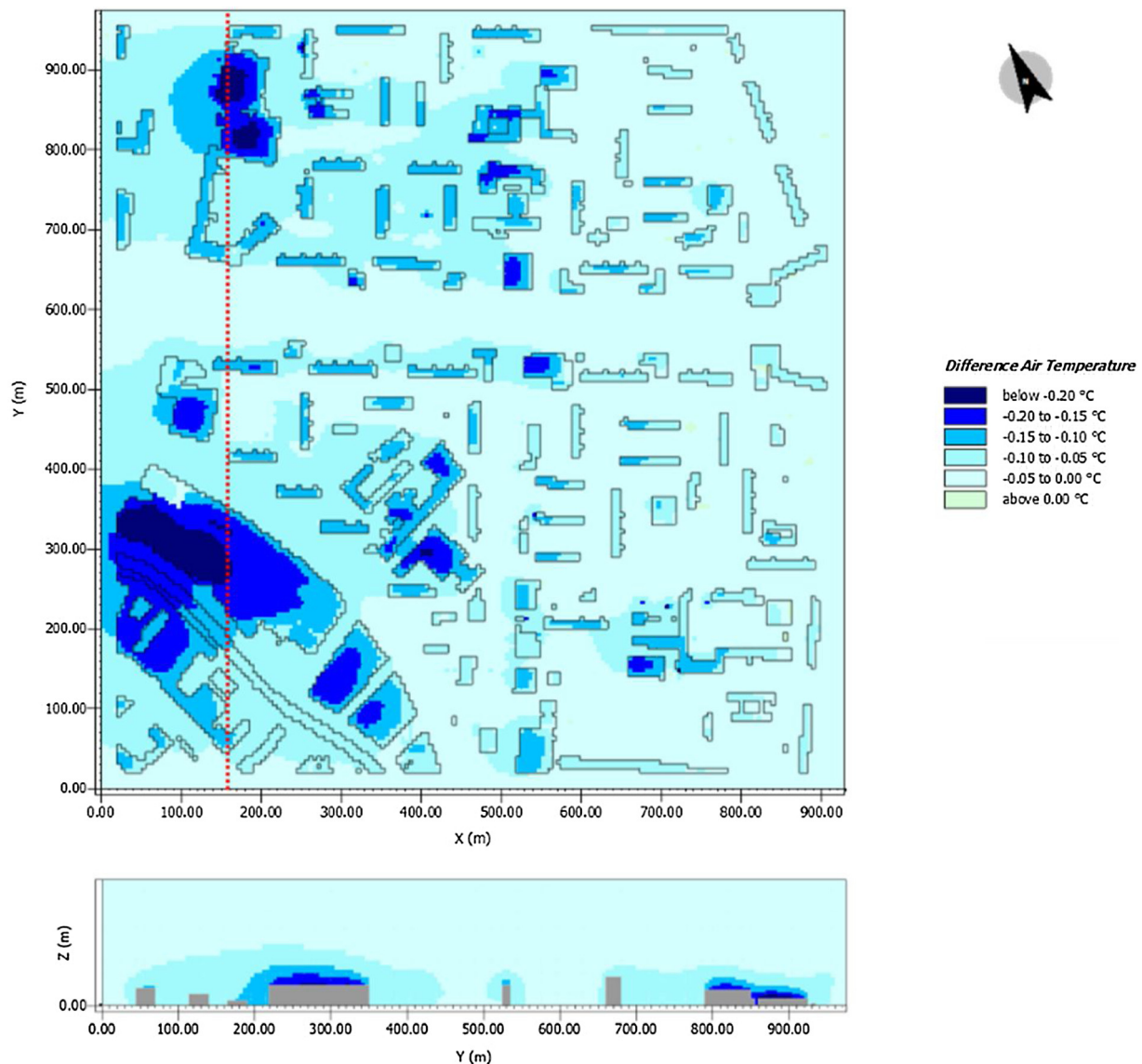
Fig. 5. Air temperature ( T_a ) difference between the intensive green roof scenario and the baseline scenario ( T_{a_{IGR}} - T_{a_{base}} ) at 14:00 CET (top) for the whole KMA area and (bottom) along y-profile at x = 157 m (marked by red dotted line). (For interpretation of the references to colour in this figure legend, the reader is referred to the web version of this article.)
