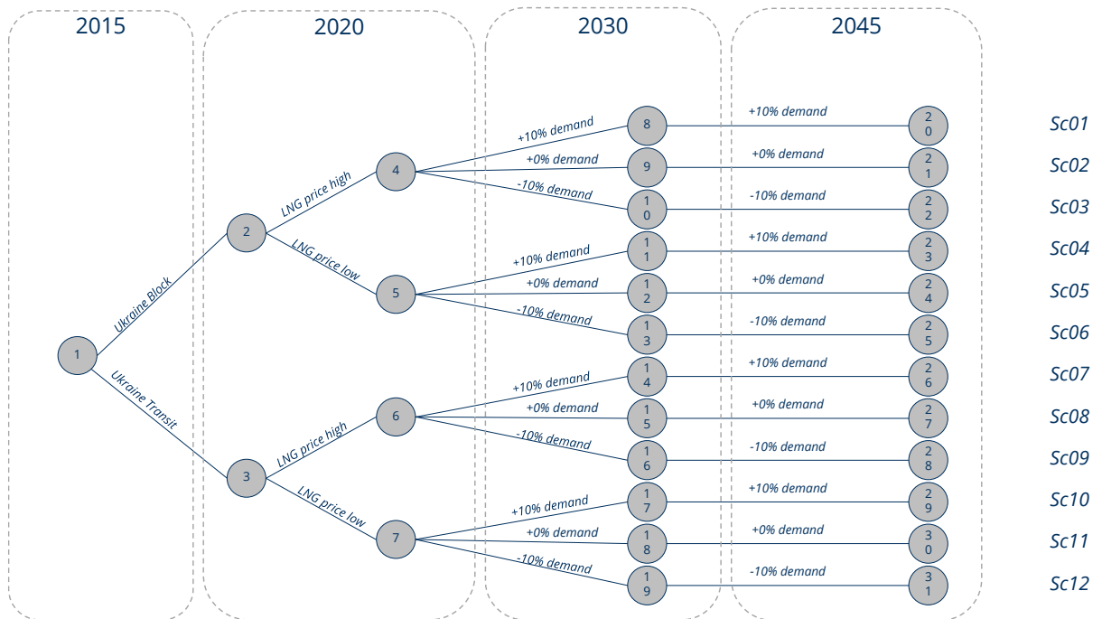
Figure 7: Scenario tree.
