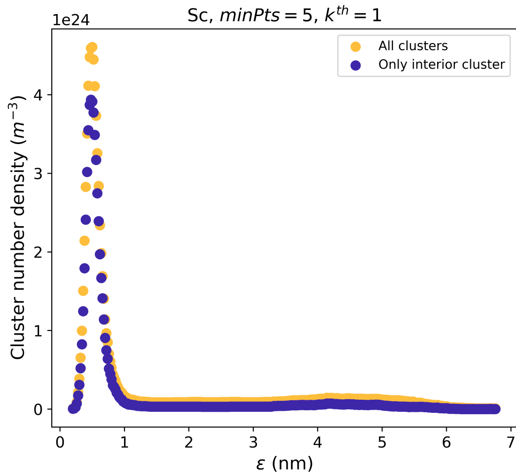
Figure 7: What are the number of clusters per unit volume, quantified using high-throughput studies of the DBScan/maximum separation clustering parameter?
