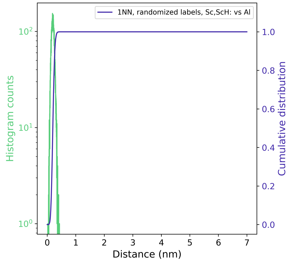
Figure 8: What is the kth nearest neighbor distribution function for particular ion types about specific ion types?
