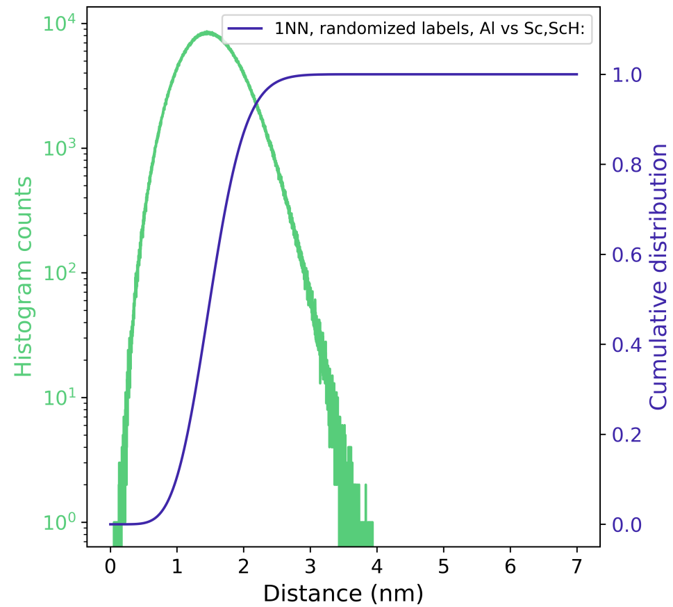
Figure 6: What is the kth nearest neighbor distribution function for particular ion types about specific ion types?
