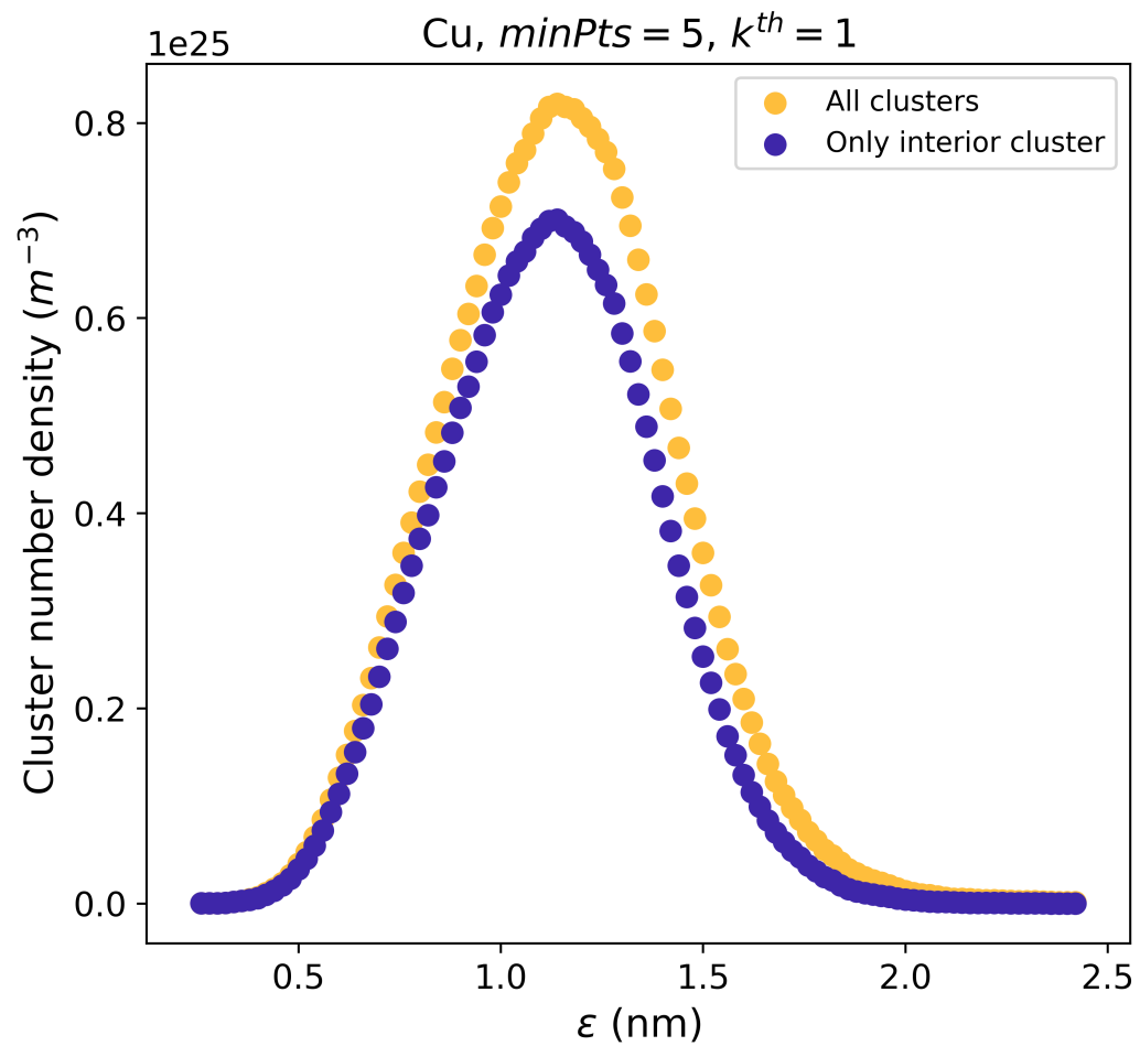
Figure 16: What are the number of clusters per unit volume, quantified using high-throughput studies of the DBScan/maximum separation clustering parameter?
