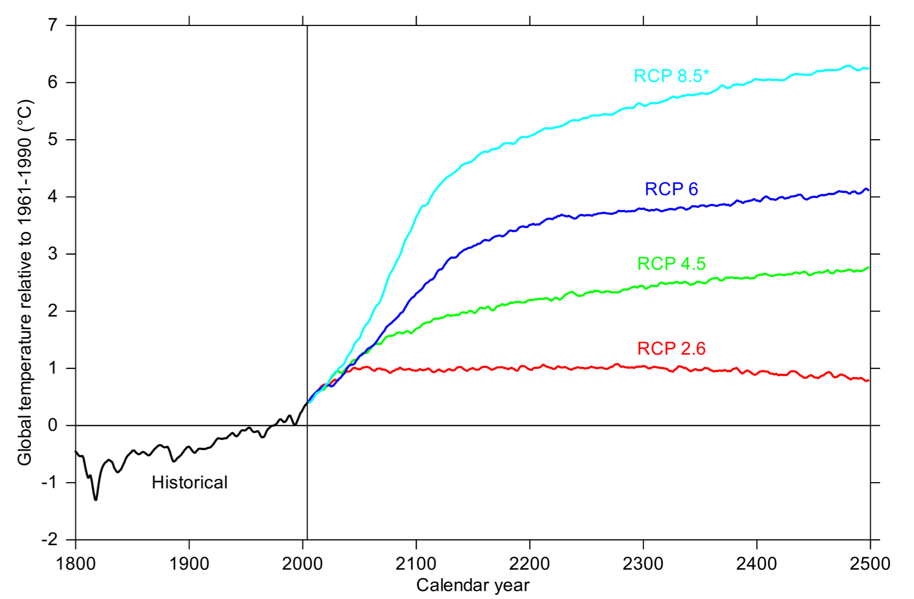
The simulated changes in global temperature for each scenario, using a global climate model.
