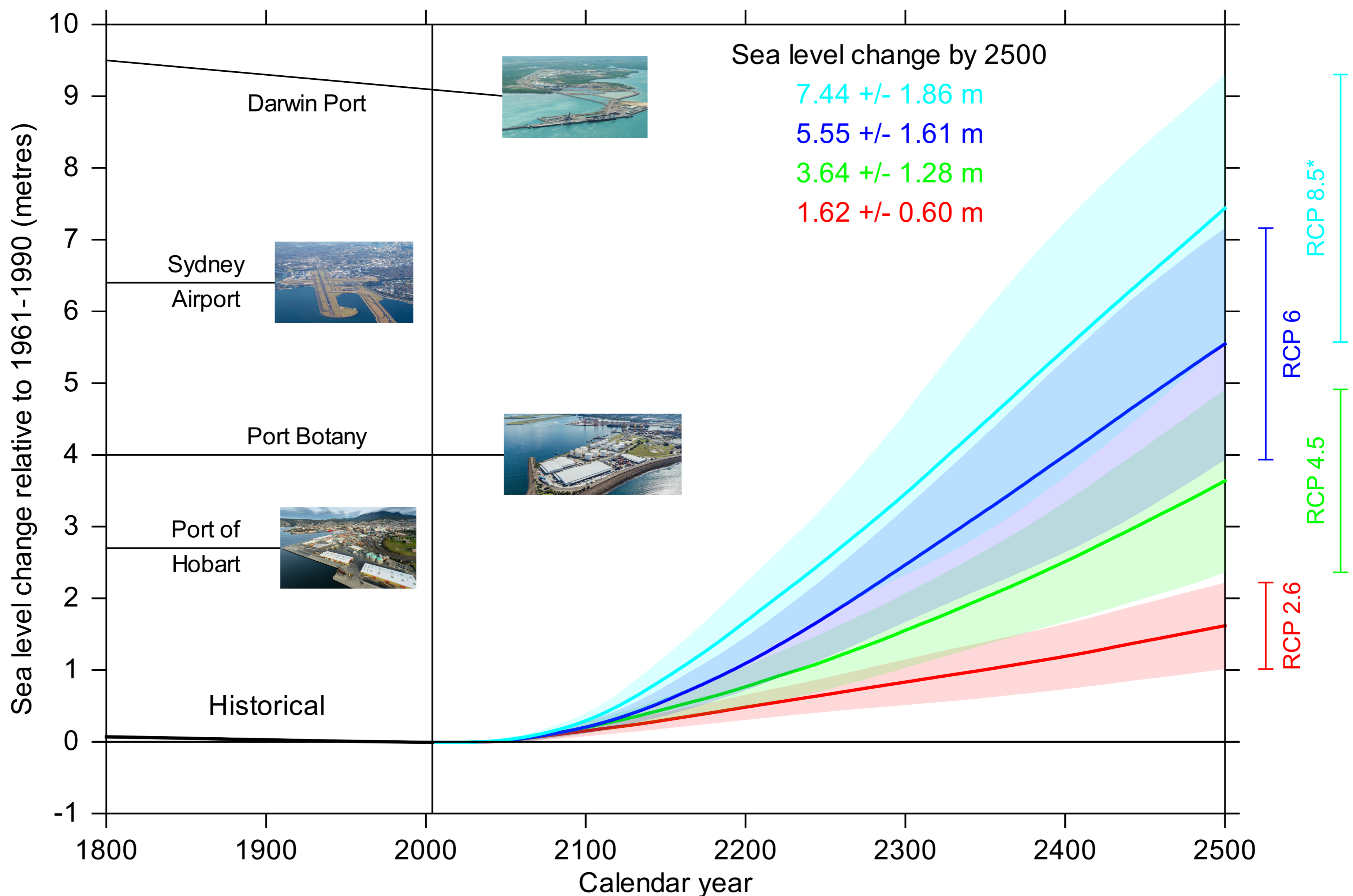
The simulated contribution of the Antarctic Ice Sheet to global sea level for each scenario, using different plausible ice sheet models. 90% of model estimates lie within the shaded ranges.
