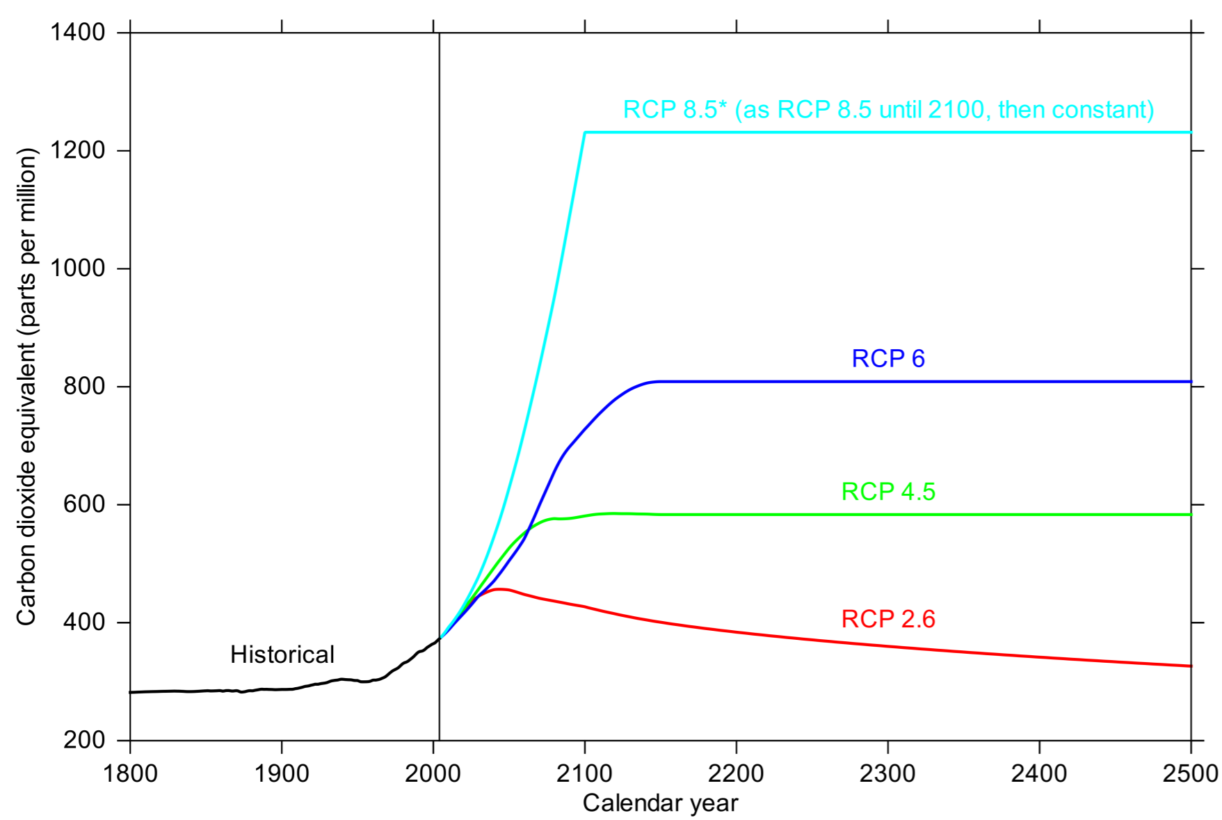
The climate scenarios studied here (as adopted by the IPCC Fifth Assessment Report).
