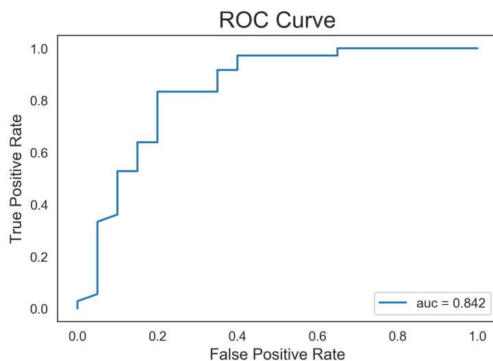
Fig. 4 The sensitivity and specificity curve (i.e., sensitivity /positive predictive value curve or, equivalently true positive rate / false positive rate as depicted in the Figure) and the area under the ROC curve.
