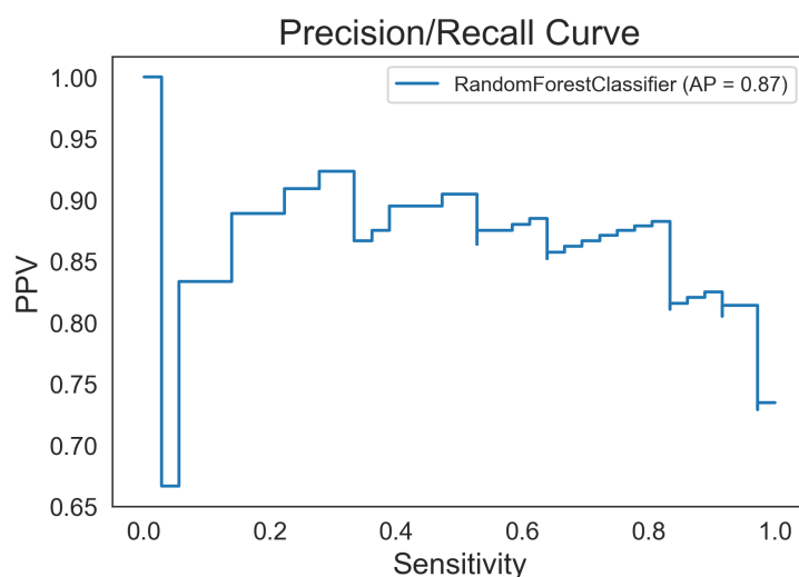
Fig. 5 The precision/recall (i.e., positive predictive value / sensitivity curve) and its area.
