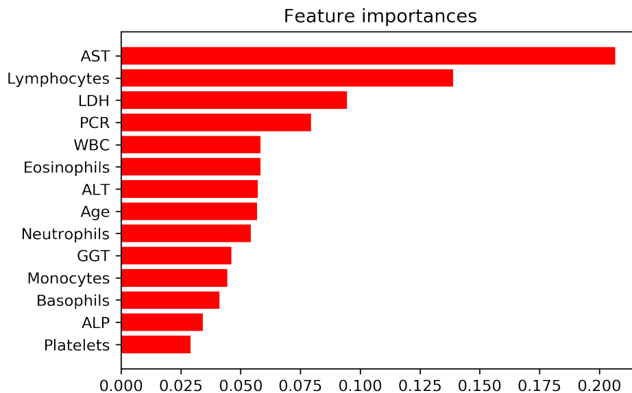
Fig. 6 Feature importance scores for the best performing model.
