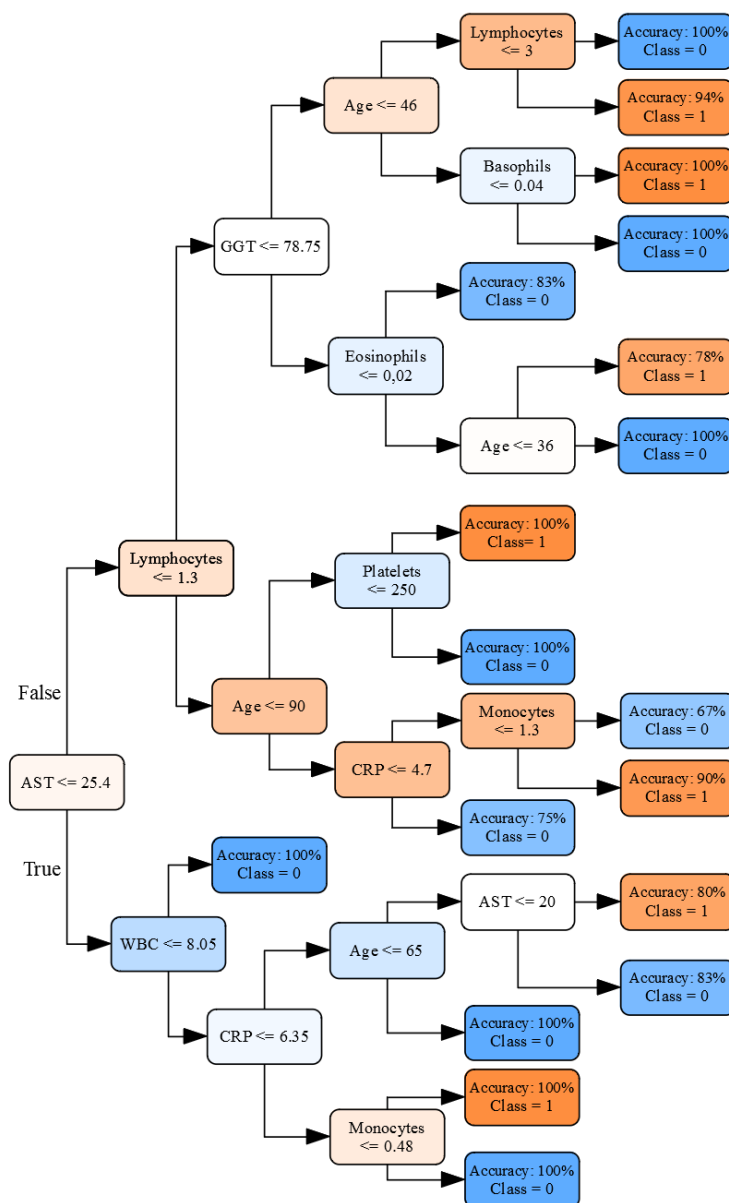
Fig. 7 An interpretable Decision Tree, developed in order to support the interpretation of the predictions from the other models. Color gradients denote predictivity for either classes (shades of blue correspond to COVID-19 negativity, shades of orange to positivity).
