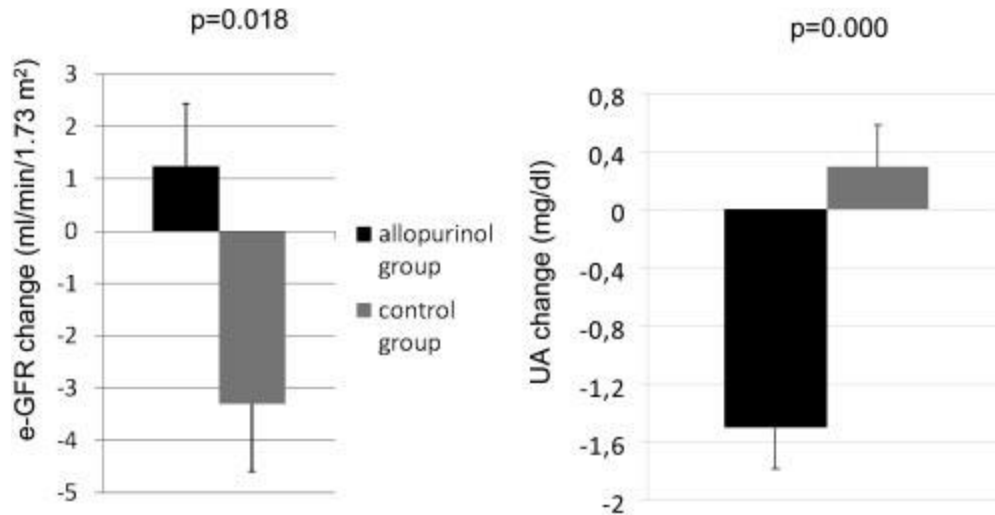
Figure 2. Change in UA levels and change in eGFR at end of research. Values are articulated as mean \pm SEM.
