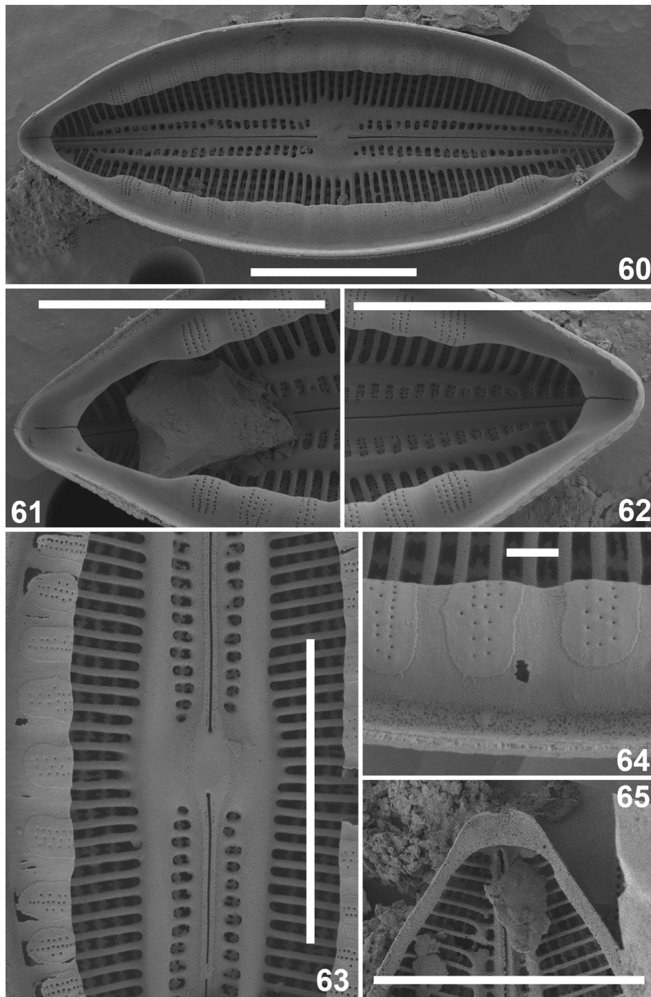
Figs 60–65. Mastogloia senegalensis Van de Vijver, Fofana, Sow & Ector sp. nov. Scanning electron micrographs (SEM) of valves from the Lac de Guiers type population ( Van de Vijver sample SEN-42 ). 60. SEM internal view of an entire valve with the partectal ring. 61–62. SEM internal details of the partectal ring near the valve apices showing the cleft on each apex. 63. SEM internal detail of the central area and part of the partectal ring. 64. SEM internal detail of the partecta showing the partectal walls with 2–4 series of small, rounded pores loosely aggregated in distinct plaques. 65. SEM internal view of a valve apex without the partectal ring (note the small pseudoseptum). Scale bars: 60–63, 65 = 10 μm; 64 = 1 μm.
