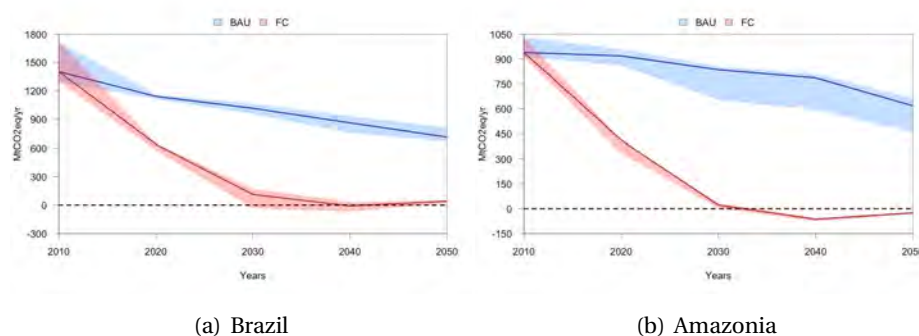
Figure 50: Net CO 2 emissions from land-use change and forestry in MtCO 2 e/yr for Brazil and Amazonia for BAU and FC scenarios. The solid line represents the median value and the shadow represents the range defined by the minimum and maximum values.
