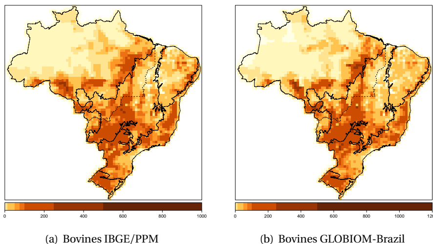
Figure 36: Spatial distribution of bovines (IBGE/PPM (a) and GLOBIOM-Brazil (b)) for 2010.
