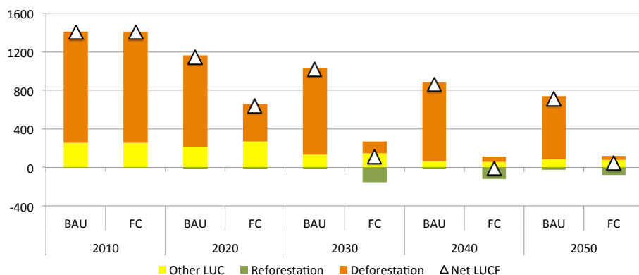
Figure 49: GHG emissions in Brazil from land-use change for different scenarios.
