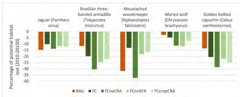
Figure 58: Impact of the policy scenarios on five different species. The five species were selected to illustrate the variability in impact between species.
