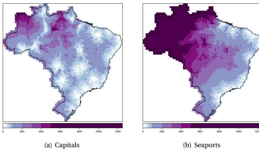
Figure 19: Transportation costs in BRL per ton to the nearest state capital (a) and to nearest seaport (b). Light blue means lower costs and purple means higher costs.
