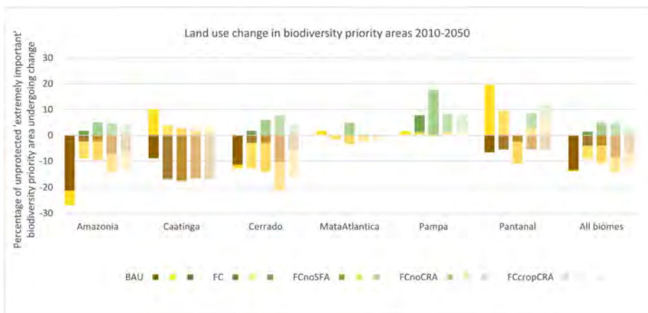
Figure 52: Projected change in area of mature forest (browns), natural land (yellows) and reforested land (greens) within unprotected biodiversity priority areas in each biome under different scenarios.
