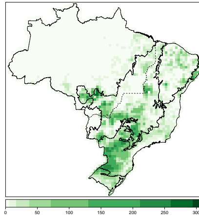
(b) Crop GLOBIOM-Brazil
