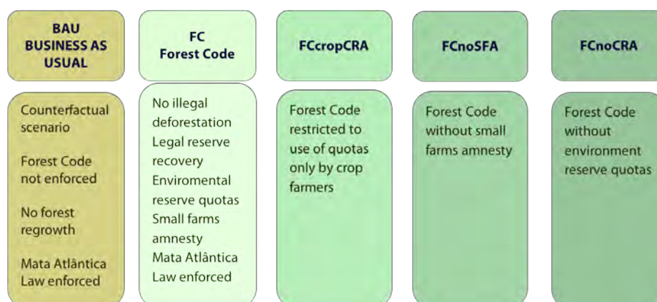
Figure 30: GLOBIOM-Brazil scenarios.
