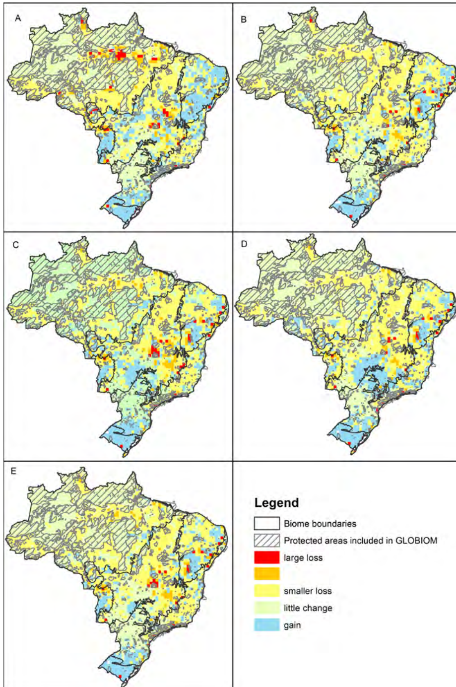
Figure 59: Map of combined species habitat change under the different scenarios: (a) BAU; (b) Forest Code; (c) FC without the small farms amnesty (FCnoSFA); (d) FC without the environmental reserve quotas (FCnoCRA); and (e) FC with the quota being used only by crop farmers (FCcropCRA). The maps show the combined impact of land use change on biodiversity, considering both losses in a large proportion of a species' habitat and where land use change harms a large number of species. Potential gains in the Pampa and Caatinga need to be interpreted with caution. Changes from cropland to 'natural land', due to agricultural production becoming unprofitable, do not necessarily improve habitat needs of species, since it takes time for species to recolonise areas.
