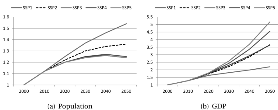
Figure 22: Growth projections for (a) population, and (b) GDP per capita in Brazil until 2050
