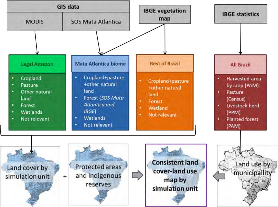
Figure 10: Creating a consistent land cover-land use map for Brazil.
