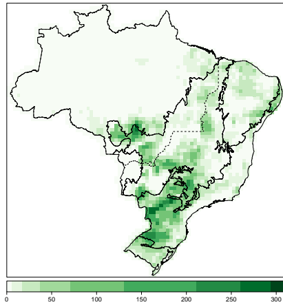
(a) Crops IBGE/PAM
