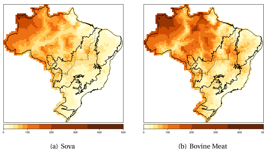
Figure 20: Combined transportation costs in US$ per ton for (a) soybeans and (b) bovine meat)
