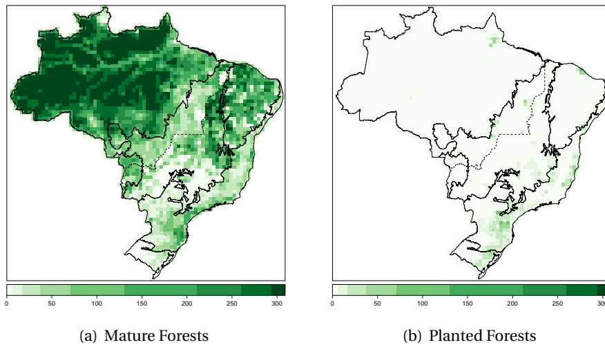
Figure 17: Final land cover map with areas of (a) forest and (b) planted forests. Values are in thousand of hectares per 50 \times 50 \text{ km}^2 cell.
