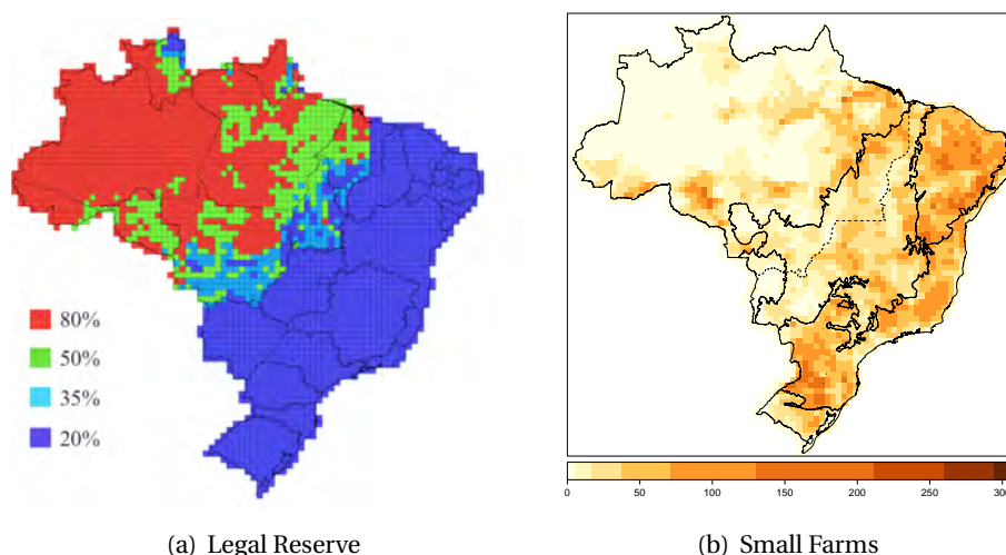
Figure 28: Legal Reserve percentages (a) and area of small farms (b) per simulation unit.
