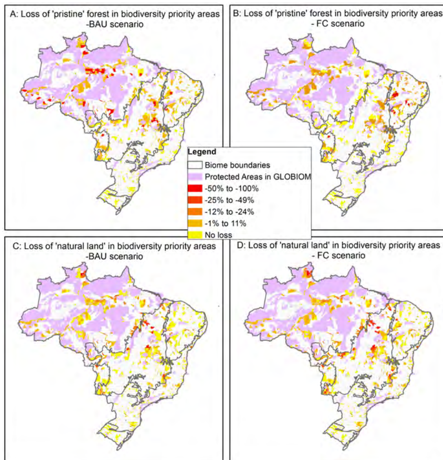
Figure 53: Change in mature forest (upper panels) and natural land (lower panels) in Brazil's biodiversity priority areas under two different scenarios: (A and C) business as usual, BAU; (B and D) forest code, FC. Protected areas are also highlighted. These areas are likely to be important for biodiversity but do not change in the simulations.
