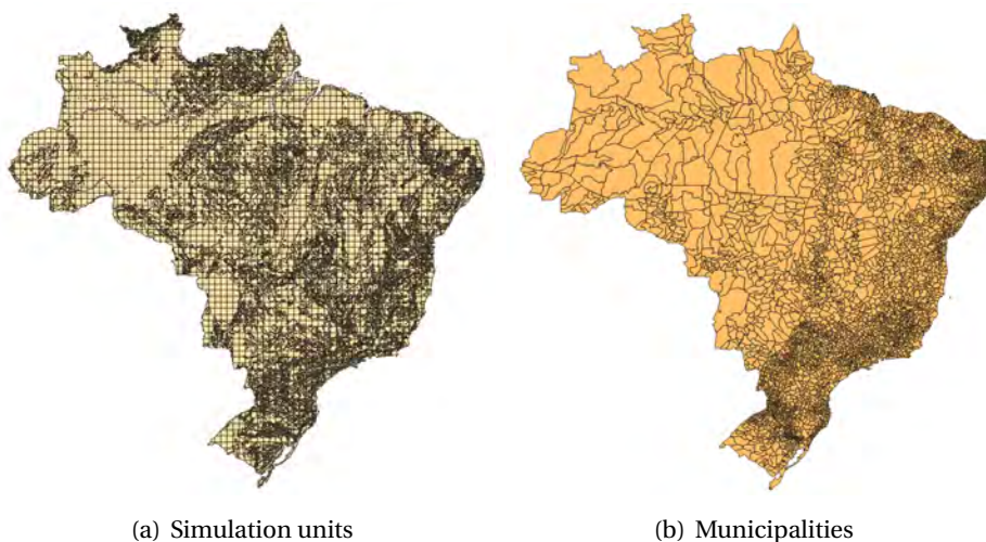
Figure 3: Simulation units (a) and municipalities (b) of Brazil.
