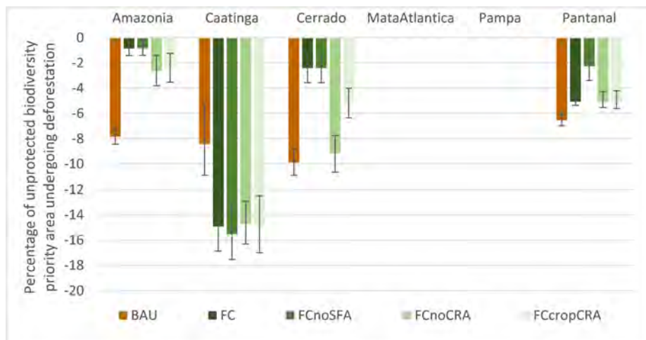
Figure 54: Variation in deforestation projected to occur in unprotected biodiversity priority areas; for each biome the bars represent different scenarios and the error bars show uncertainty due to local allocation.
