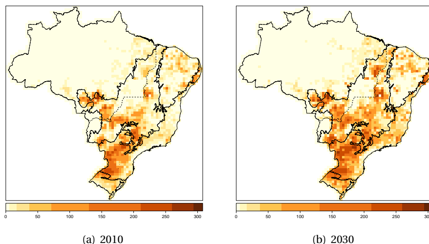
Figure 44: Spatial distribution of cropland projected for 2010 and 2030 in the FC scenario. Values are thousands of ha per 50 x 50 km 2 cell.
