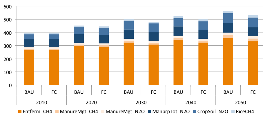
Figure 51: GHG emissions in Brazil from crop and livestock for different scenarios.
