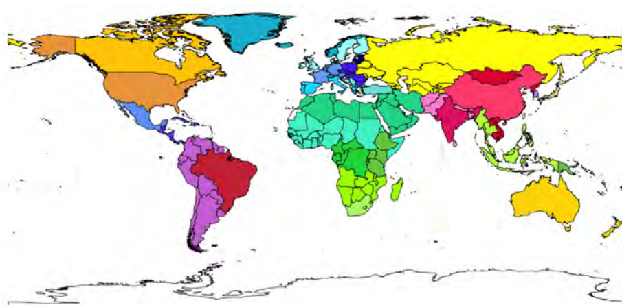
Figure 26: The 30 regions that can trade with each other in GLOBIOM.
