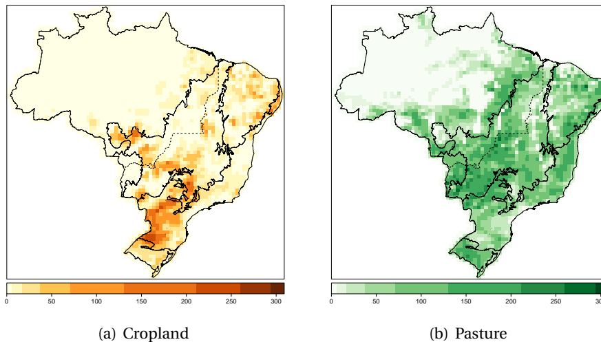
Figure 16: Final land cover map with areas of (a) crops (b) pasture. Values are in thousand of hectares per 50 x 50 km 2 cell.
