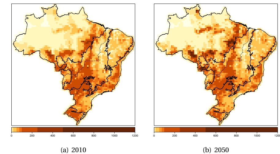
Figure 46: Spatial distribution bovine heads in 2010 and 2050 for FC scenario. Values are thousands of tropical livestock units (TLUs) per 50 x 50 km 2 cell.
