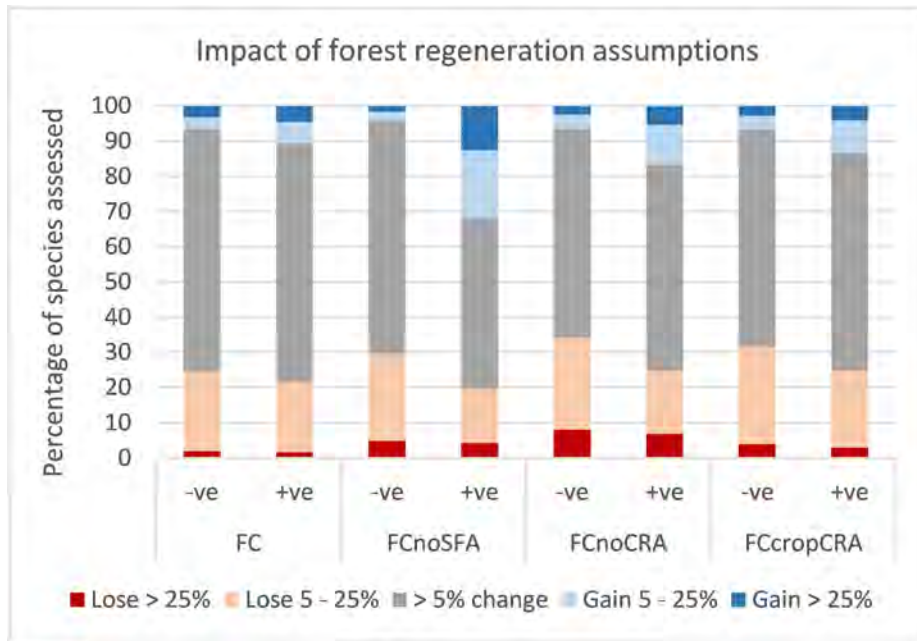
Figure 57: Variation in the impact of land use change on species depending on how forest regeneration happens. For each scenario, the left hand bar is the case when regenerated areas are not suitable for forest species (-ve) and the right hand bar represents the opposite assumption (+ve).
