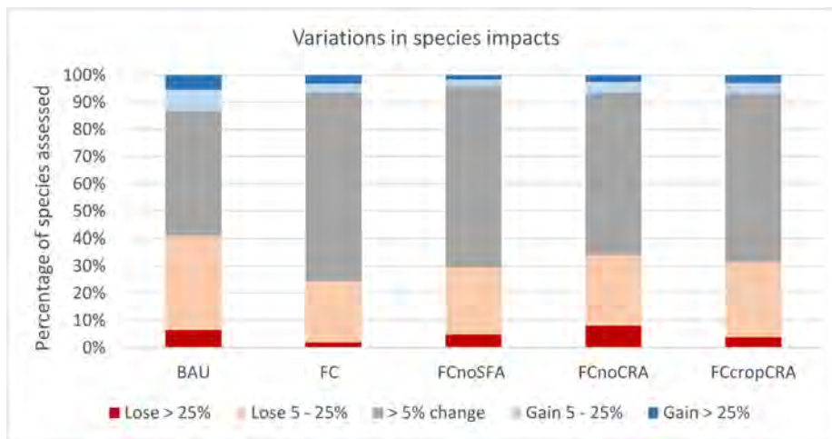
Figure 56: Impacts on species of modelled land use change under five scenarios, expressed as percentage of the assessed species projected to experience different degrees of net change in extent of potential habitat.
