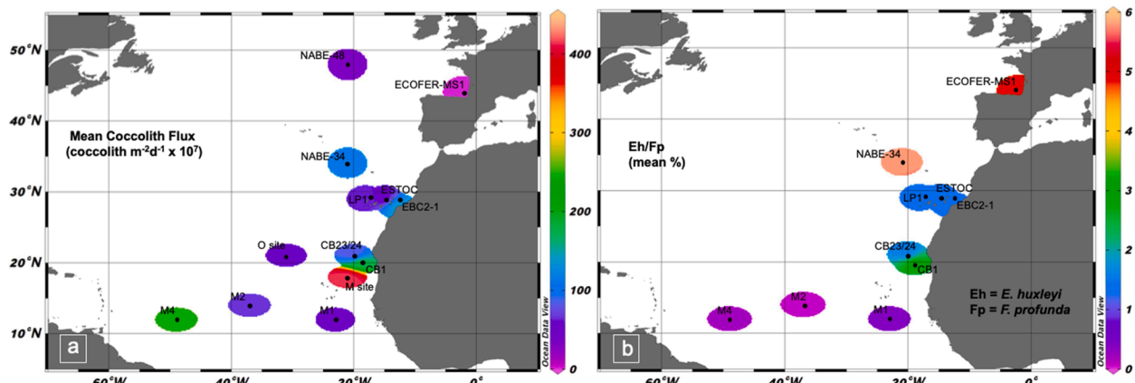
Fig. 9. Comparison between the (a) mean coccolith fluxes ( \text{coccolith m}^{-2}\text{d}^{-1} ) and (b) ratio between the mean percentages of E. huxleyi and of F. profunda presented in this study and from other sediment trap studies undertaken in the North Atlantic: NABE-48 and NABE-34 (April 1989 to April 1990) from Broerse et al. (2000), LP1, ESTOC and EBC2-1 (January to September 1997) from Sprengel et al. (2002), ECOFER-MS1 (June 1990 to August 1991) from Beaufort and Heussner (1999), CB1 (March 1988 to March 1989) from Köbrich and Baumann (2009), O site and M site (February 1991 and November 1992) from Bory et al. (2001), M2 and M4 from Guerreiro et al. (2017) and CB and M1 from this study. For NABE-48, O site and M site, there are no data available for both species, whereas for LP1, ESTOC and EBC2-1 Sprengel et al. (2002) only provide mean percentages for all three sites.
