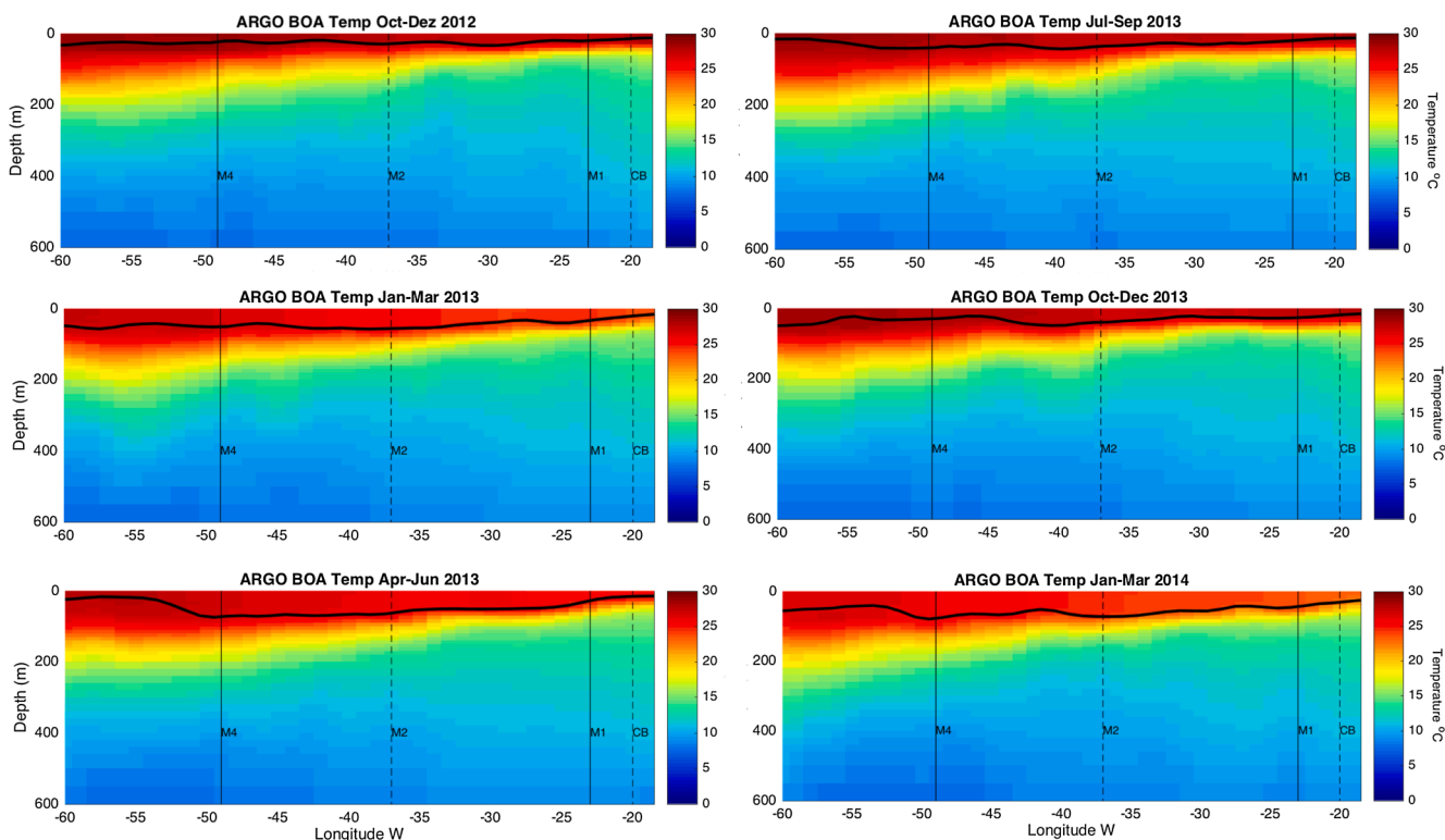
Fig. 3. Transatlantic depth profiles of temperature ( ^\circ\text{C} ) and mixed layer depth (MLD, black line) along \sim 12^\circ\text{N} , from October 2012 to March 2014, obtained from in situ Argo-BOA data (Li et al., 2017; see Section 3.3).
