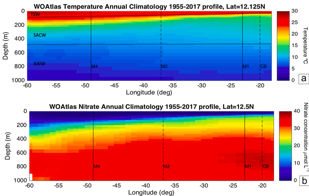
Fig. 2. Transatlantic depth profiles of temperature (a) and nitrate concentrations (b) along \sim 12^\circ\text{N} , from 1955 to 2017 (World Ocean Atlas; Locarnini et al., 2013; Garcia et al., 2014, respectively). Main water masses (a) are the tropical surface water (TSW), South Atlantic Central Water (SACW) and Antarctic Intermediate Water (AAIW) based on Emery and Meincke (1986), Reid (1994), and Stramma and England (1999). Sediment trap moorings M2 (at 14^\circ\text{N} ) and CB (at 21^\circ\text{N} ) located north of 12^\circ\text{N} are indicated by dashed vertical lines, whereas M4 and M1 (at 12^\circ\text{N} ) are indicated by solid vertical lines.
