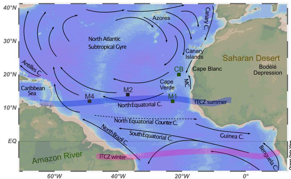
Fig. 1. Location of the sediment trap mooring sites (squares) and main surface currents (arrows) in the equatorial Atlantic Ocean, including the Mauritanian Current (MC) flowing northwards off NW Africa (adapted from Mann and Lazier, 2006; Pelegrí et al., 2017). New time-series from CB and M1 in the eastern tropical North Atlantic are indicated by green squares, with previously published data from M2 and M4 (Guerreiro et al., 2017) given in dark grey. Schematic representation of the seasonal migration of the Intertropical Convergence Zone according to Basha et al. (2015). (For interpretation of the references to colour in this figure legend, the reader is referred to the web version of this article.)
