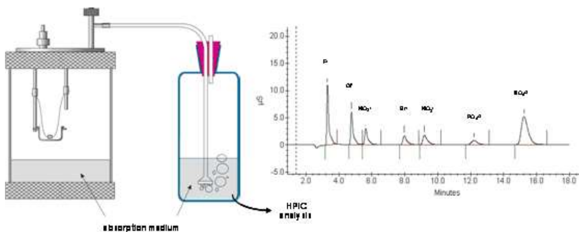
Figure 26. Biomass preparation for Cl, and S analysis via HPIC chromatography (absorption medium: Na 2 CO 3 /NaHCO 3 buffer, pH= 9.5).
