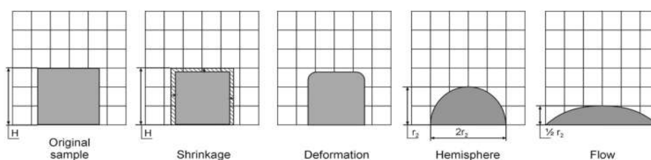
Figure 27 Key temperatures in the ash melting process.
