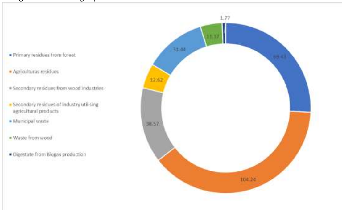
Figure 25. Biomass repartition per typology in terms of energy available (MTOE)
