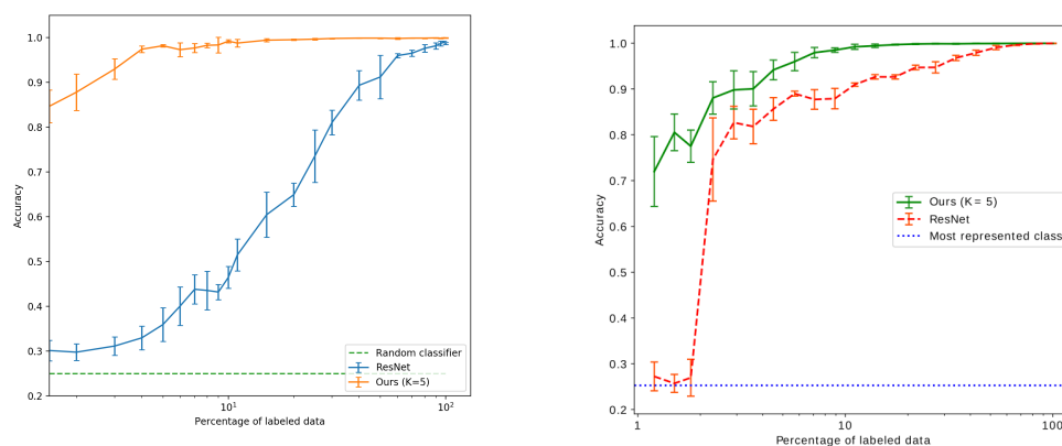
Figure 1. Reproduction of Figure 4 from the original article (right). The same striking difference between ResNet and the authors’ method is observed when training on a limited amount of labeled data.
