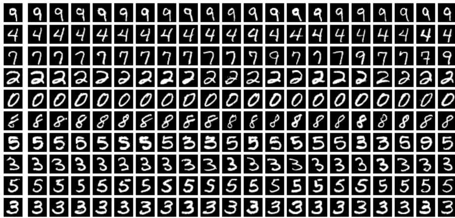
(a) MNIST
