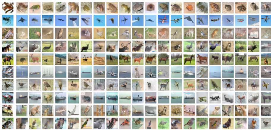
(b) CIFAR-10
