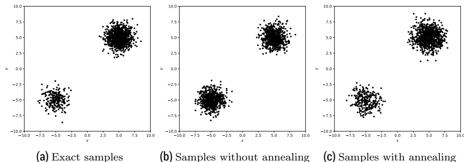
Figure 3. Effect of low-density regions on sampling with Langevin dynamics.
