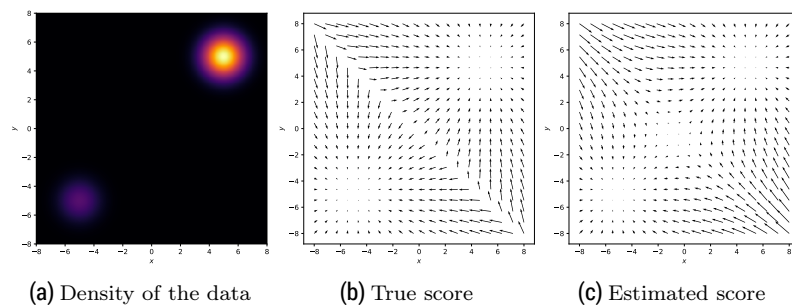
Figure 2. Effect of low-density regions on score estimation.
