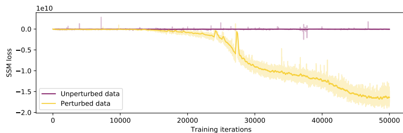
Figure 1. Loss curves for score networks trained on CIFAR-10 before and after data perturbation.
