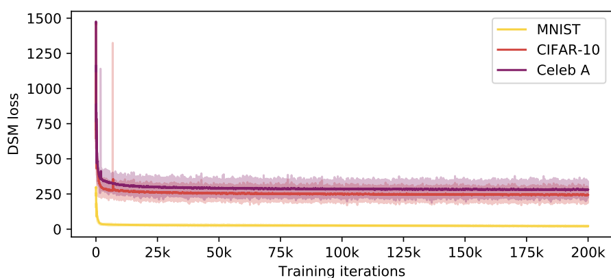
Figure 12. Loss curves for training real model
