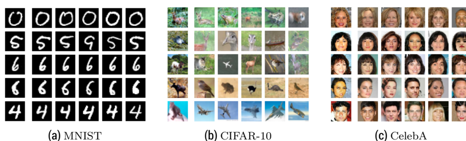
Figure 6. k = 5 nearest neighbours from the training data for 5 samples based on l_2 -distance.
