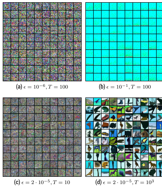
Figure 8. Samples from the best CIFAR-10 model with different values of \epsilon and T .
