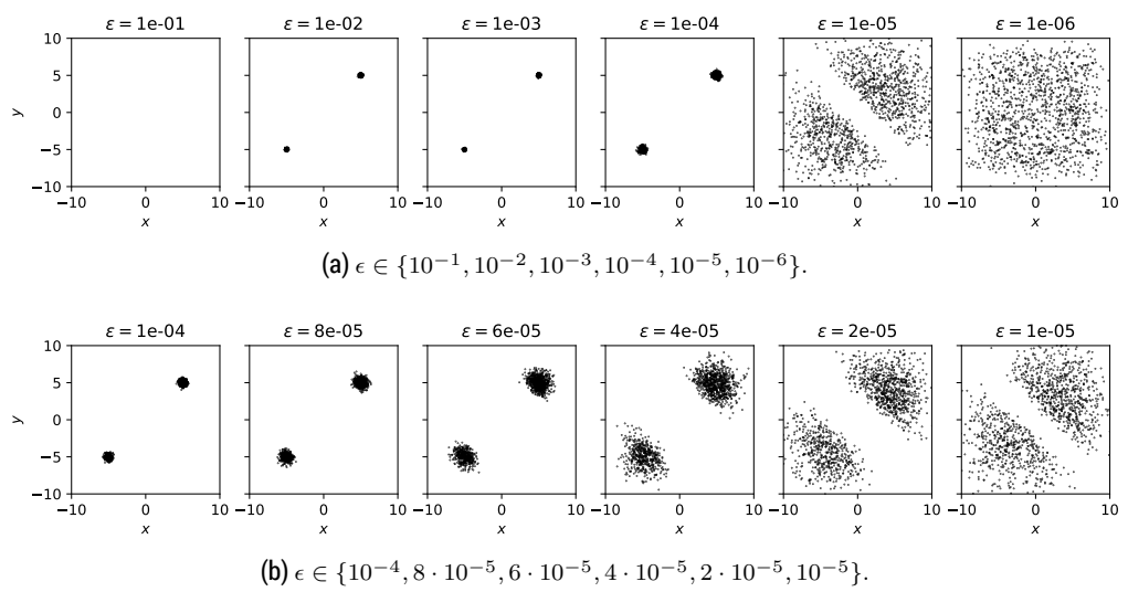
Figure 11. Samples obtained with different values of \epsilon for toy data with annealed Langevin dynamics. Even after expanding the search in the promising interval \epsilon \in \{10^{-4}, 10^{-5}\} , we did not find a value of \epsilon yielding satisfying results.
