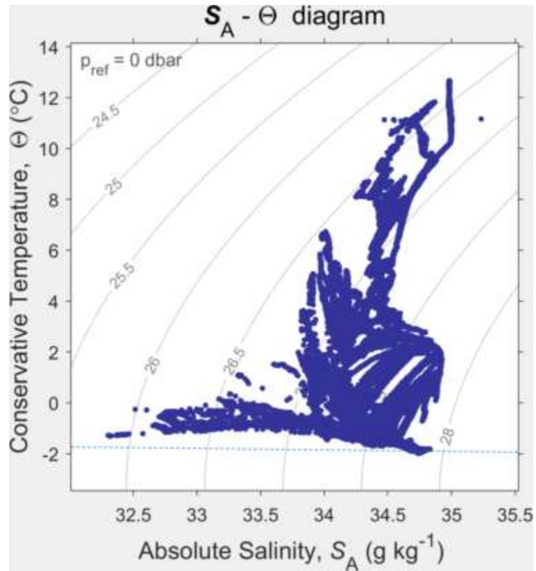
Figure 4: Absolute salinity versus conservative temperature diagram from all ACE CTD stations. Blue dots are single CTD data values, gray contours show the density anomalies (+1000 kg/m 3 ), and the dotted line shows the freezing line. The figure was created using the TEOS-10 GSW toolbox ( http://www.teos-10.org/pubs/gsw/html/gsw_contents.html ).
