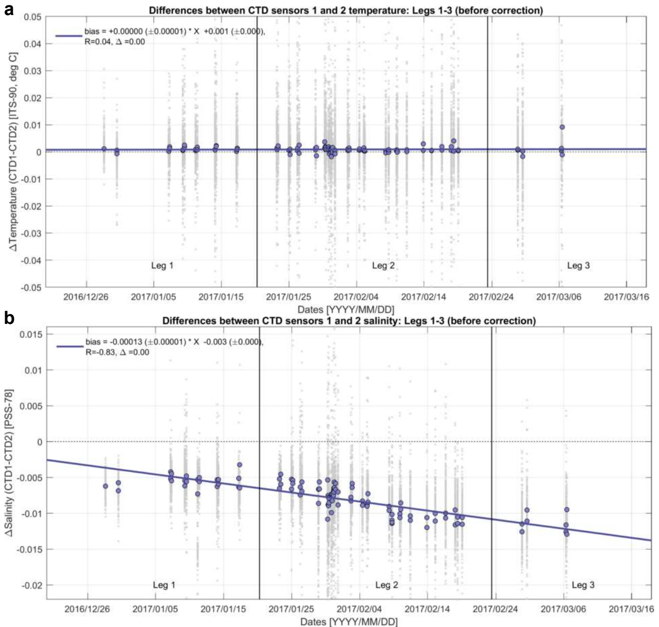
Figure 1: CTD temperature and salinity comparison between sensors 1 and 2 (before corrections). (a) In-situ temperature difference of CTD sensors. (b) Practical salinity difference of CTD sensors. The difference shows the value of sensor 1 minus the value of sensor 2. Note that all values are shown before any post-cruise correction has been applied. Each panel shows single data points (gray crosses), averages of one cast (blue dots), and linear regression lines of these averages (blue lines). The result of the regression analysis is displayed in the figure legend. Data is only shown when both sensors are available. Vertical black lines denote the end of legs 1 and 2, respectively. Note that only sensor 1 is being published in the final data set, due to a failure of sensor 2 during leg 3 and missing post-cruise calibration values for sensor 2.
