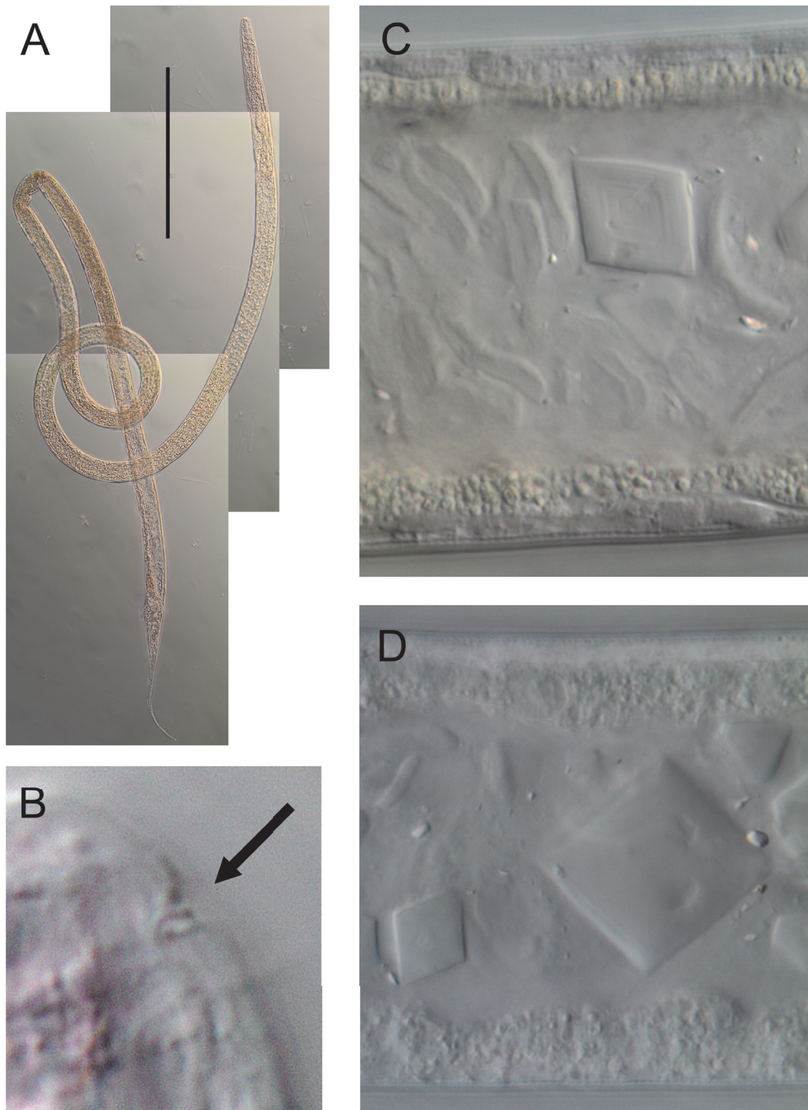
Fig. 3. Thelonema clarki sp. nov. Light micrographs. A. Holotype, ♂, entire body. B. Cross-section view of sunken papilla, second circle of cephalic sensillae. C. Female gut content, showing crystalline structures and other unidentified contents. D. Juvenile gut showing crystalline structures. Arrow shows position of sunken papilla of third circle of cephalic sensillae. Scale bar: A = 520 \mu\text{m} ; B = 5 \mu\text{m} ; C–D = 20 \mu\text{m} .
