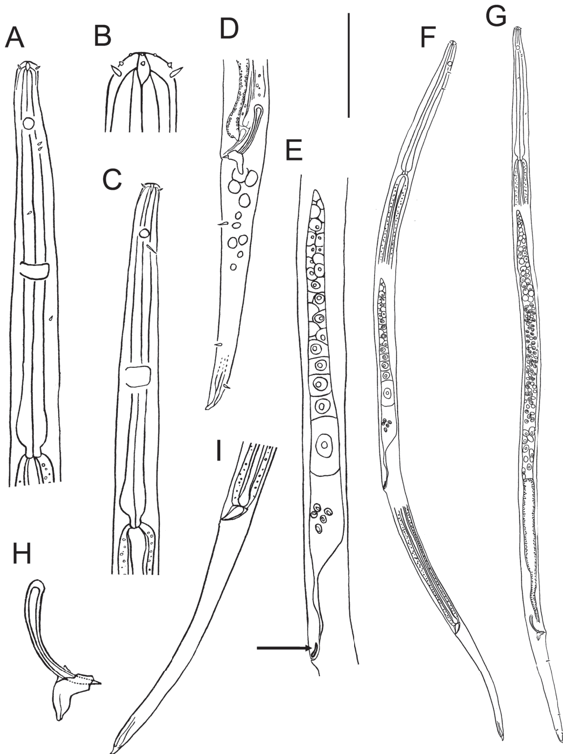
Fig. 6. Monhystrella kermadecensis sp. nov. A. Male anterior body region. B. Male head region. C. Female anterior body region. D. Male posterior body region. E. Female reproductive system. F. Entire ♀. G. Entire ♂, holotype. H. Male copulatory apparatus. I. Female posterior body region. Arrow shows position of cuticularised piece anterior to vulva. Scale bar: A, C–E, I = 25 µm; B = 7 µm; F–G = 70 µm; H = 12 µm.
