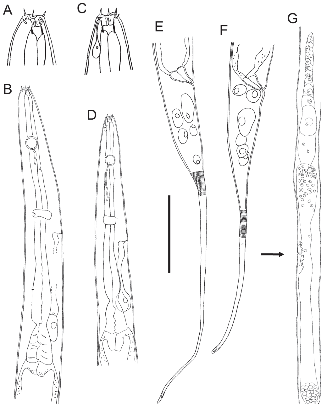
Fig. 2. Thelonema clarki sp. nov. Paratypes, ♀ and juvenile. A. Female head. B. Female anterior body region. C. Juvenile head. D. Juvenile anterior body region. E. Female posterior body region. F. Juvenile posterior body region. G. Female reproductive system. Arrow shows position of vulva. Scale bar: A–C = 40 µm; B–D = 100 µm; E–F = 90 µm; G = 210 µm.
