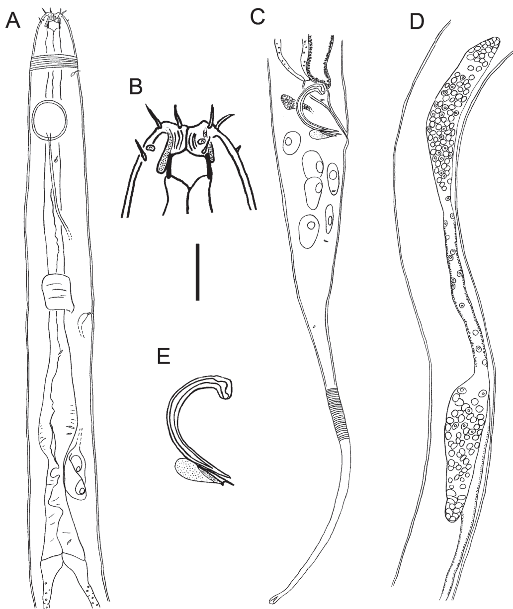
Fig. 1. Thelonema clarki sp. nov. Holotype, ♂. A. Anterior body region. B. Head, showing buccal cavity and cephalic sensillae. C. Posterior body region. D. Gonads, right-hand side view. E. Spicule and gubernaculum. Scale bar: A, C = 40 \mu m; B = 12 \mu m; D = 45 \mu m; E = 20 \mu m.
