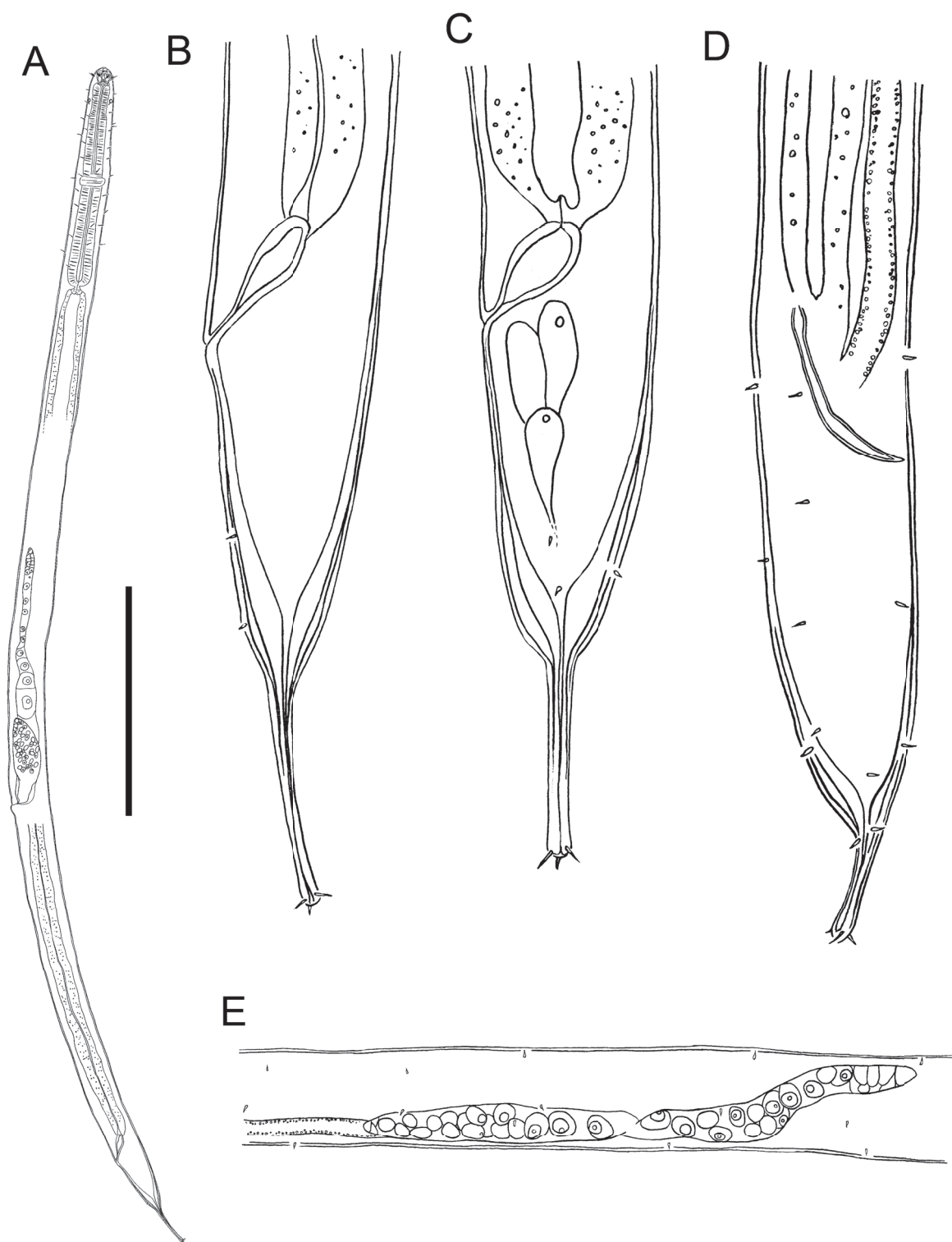
Fig. 5. Metasphaerolaimus constrictus sp. nov. A. Entire ♀. B–C. Female posterior body region. D. Male posterior body region. E. Male gonads. Scale bar: A = 300 \mu m; B–C = 55 \mu m; D = 45 \mu m; E = 80 \mu m.
